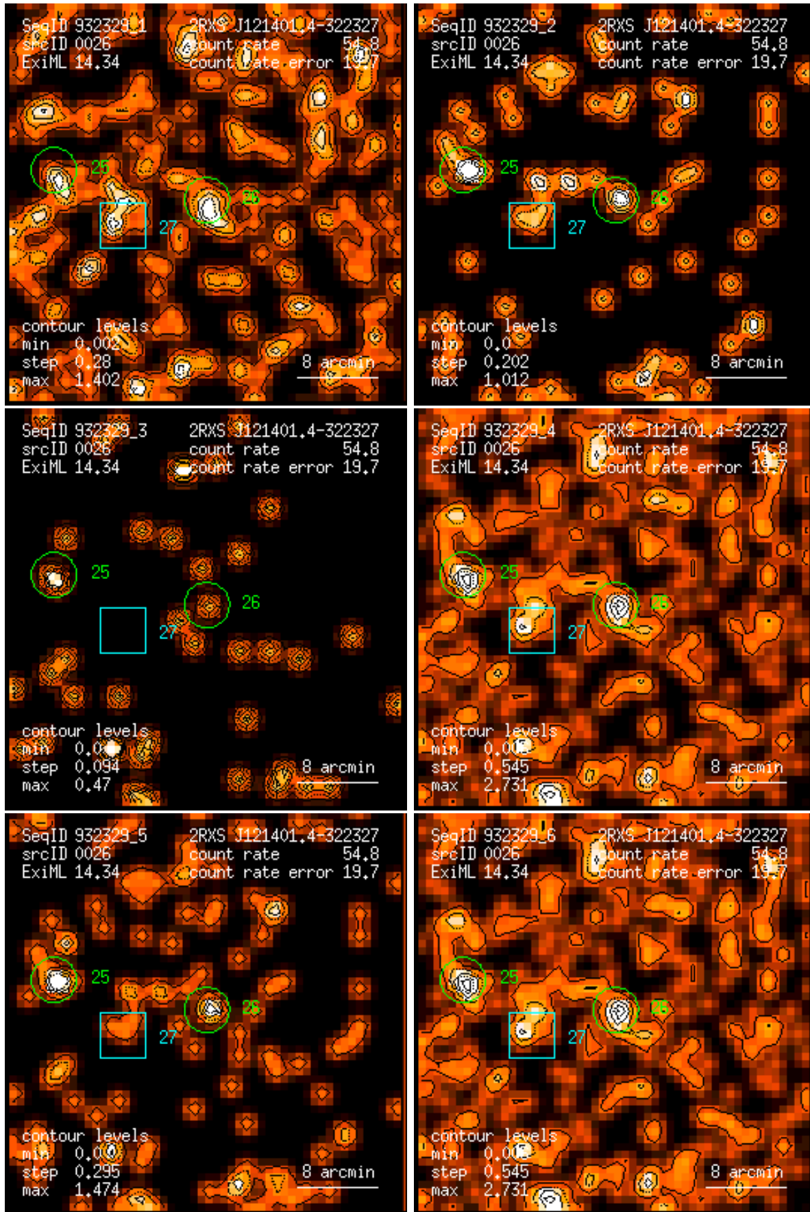
Figure 26: RASS 932329: detection 0026: band rate images, Gaussian filter: (1) PSPC channels 11 – 41, (2) 52 – 90, (3) 91 – 201, (4) 11 – 235, (5) 52 – 201, (6) 11 – 201. Broad band rates in counts/ks. Band rate contour levels in counts/ks/arcmin 2 .
