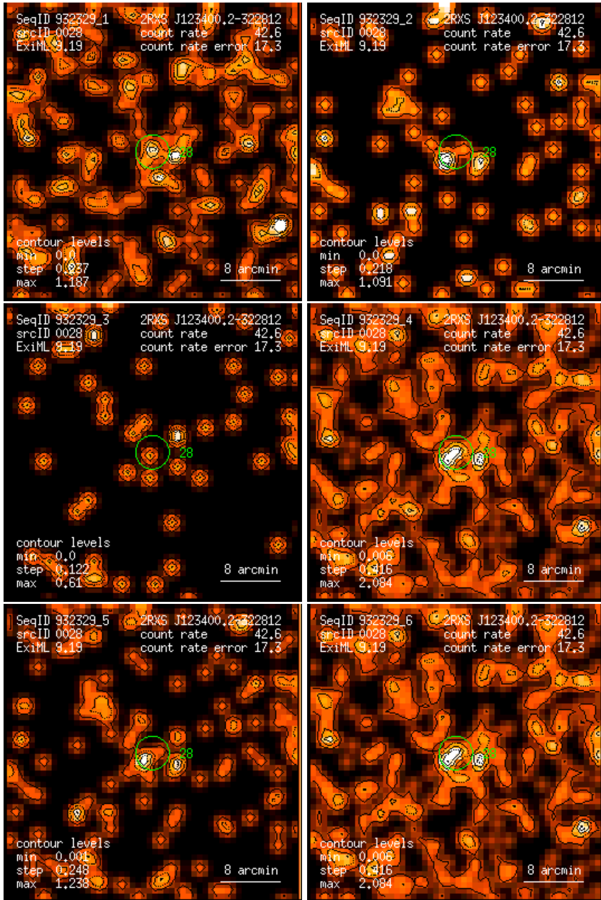
Figure 28: RASS 932329: detection 0028: band rate images, Gaussian filter: (1) PSPC channels 11 – 41, (2) 52 – 90, (3) 91 – 201, (4) 11 – 235, (5) 52 – 201, (6) 11 – 201. Broad band rates in counts/ks. Band rate contour levels in counts/ks/arcmin 2 .
