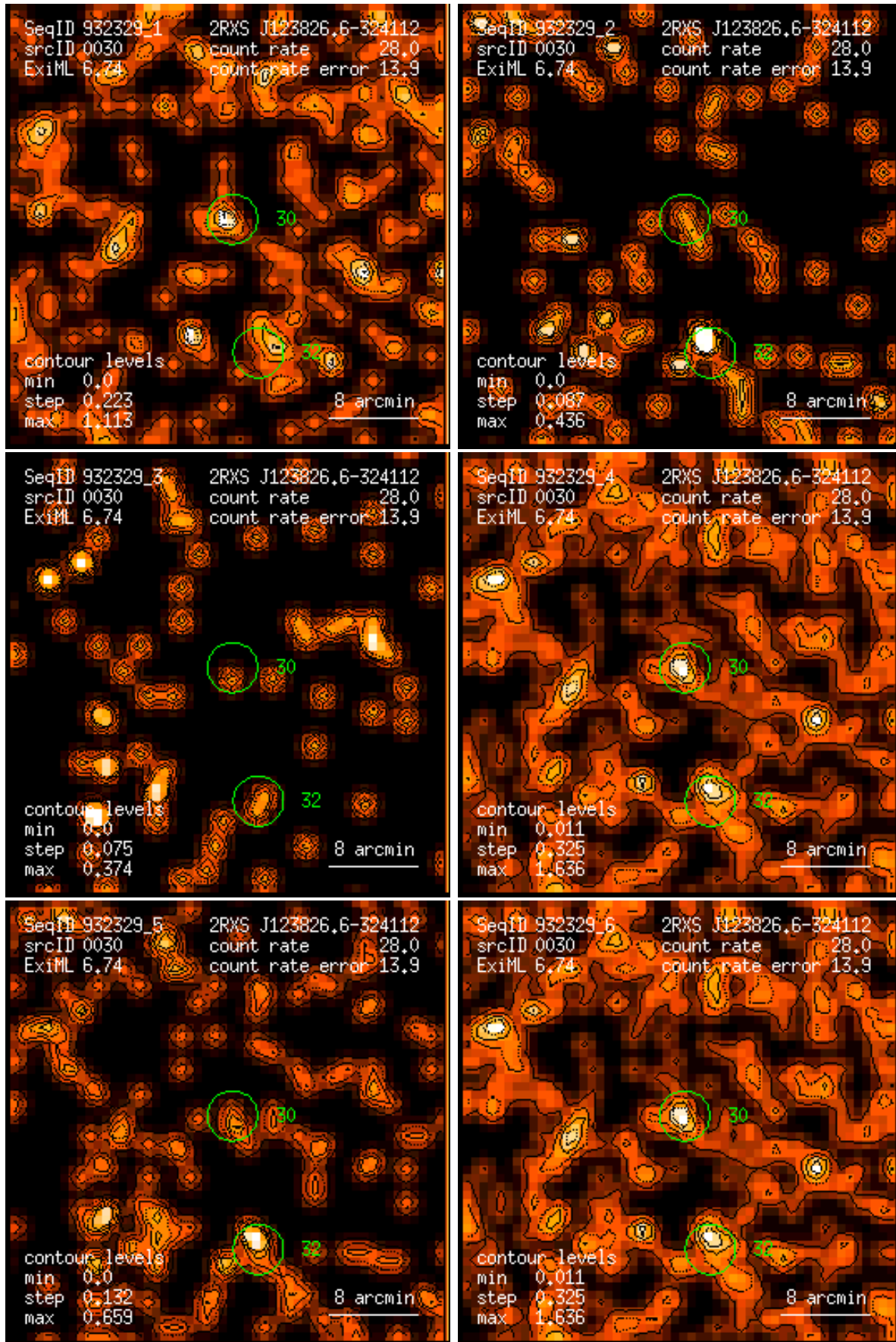
Figure 30: RASS 932329: detection 0030: band rate images, Gaussian filter: (1) PSPC channels 11 – 41, (2) 52 – 90, (3) 91 – 201, (4) 11 – 235, (5) 52 – 201, (6) 11 – 201. Broad band rates in counts/ks. Band rate contour levels in counts/ks/arcmin 2 .
