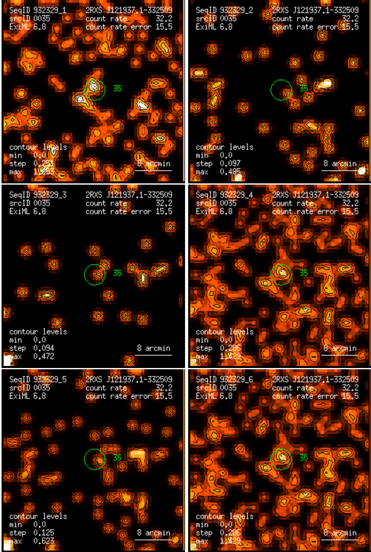
Figure 35: RASS 932329: detection 0035: band rate images, Gaussian filter: (1) PSPC channels 11 – 41, (2) 52 – 90, (3) 91 – 201, (4) 11 – 235, (5) 52 – 201, (6) 11 – 201. Broad band rates in counts/ks. Band rate contour levels in counts/ks/arcmin 2 .
