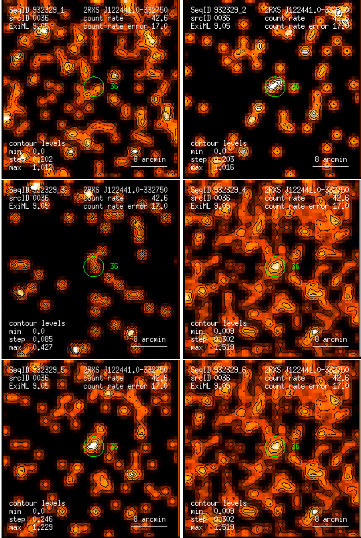
Figure 36: RASS 932329: detection 0036: band rate images, Gaussian filter: (1) PSPC channels 11 – 41, (2) 52 – 90, (3) 91 – 201, (4) 11 – 235, (5) 52 – 201, (6) 11 – 201. Broad band rates in counts/ks. Band rate contour levels in counts/ks/arcmin 2 .
