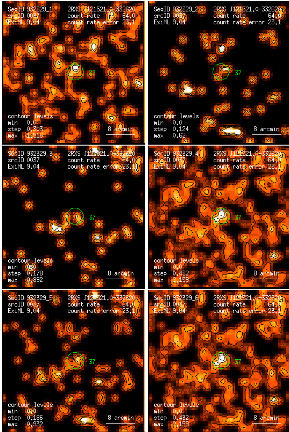
Figure 37: RASS 932329: detection 0037: band rate images, Gaussian filter: (1) PSPC channels 11 – 41, (2) 52 – 90, (3) 91 – 201, (4) 11 – 235, (5) 52 – 201, (6) 11 – 201. Broad band rates in counts/ks. Band rate contour levels in counts/ks/arcmin 2 .
