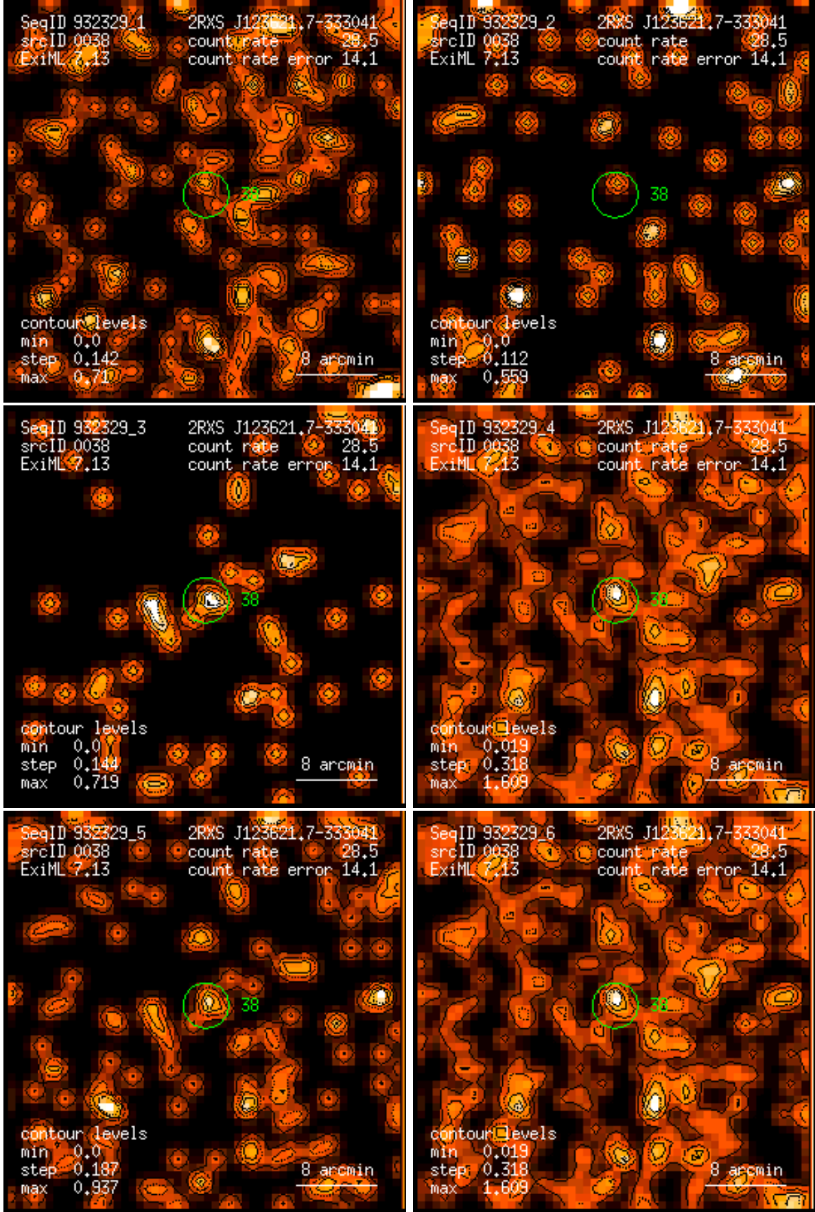
Figure 38: RASS 932329: detection 0038: band rate images, Gaussian filter: (1) PSPC channels 11 – 41, (2) 52 – 90, (3) 91 – 201, (4) 11 – 235, (5) 52 – 201, (6) 11 – 201. Broad band rates in counts/ks. Band rate contour levels in counts/ks/arcmin 2 .
