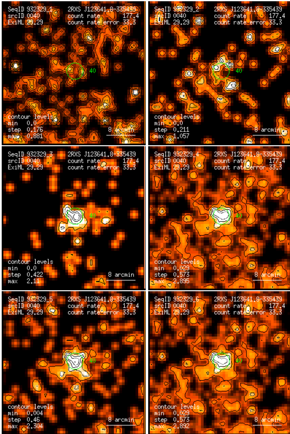
Figure 40: RASS 932329: detection 0040: band rate images, Gaussian filter: (1) PSPC channels 11 – 41, (2) 52 – 90, (3) 91 – 201, (4) 11 – 235, (5) 52 – 201, (6) 11 – 201. Broad band rates in counts/ks. Band rate contour levels in counts/ks/arcmin 2 .
