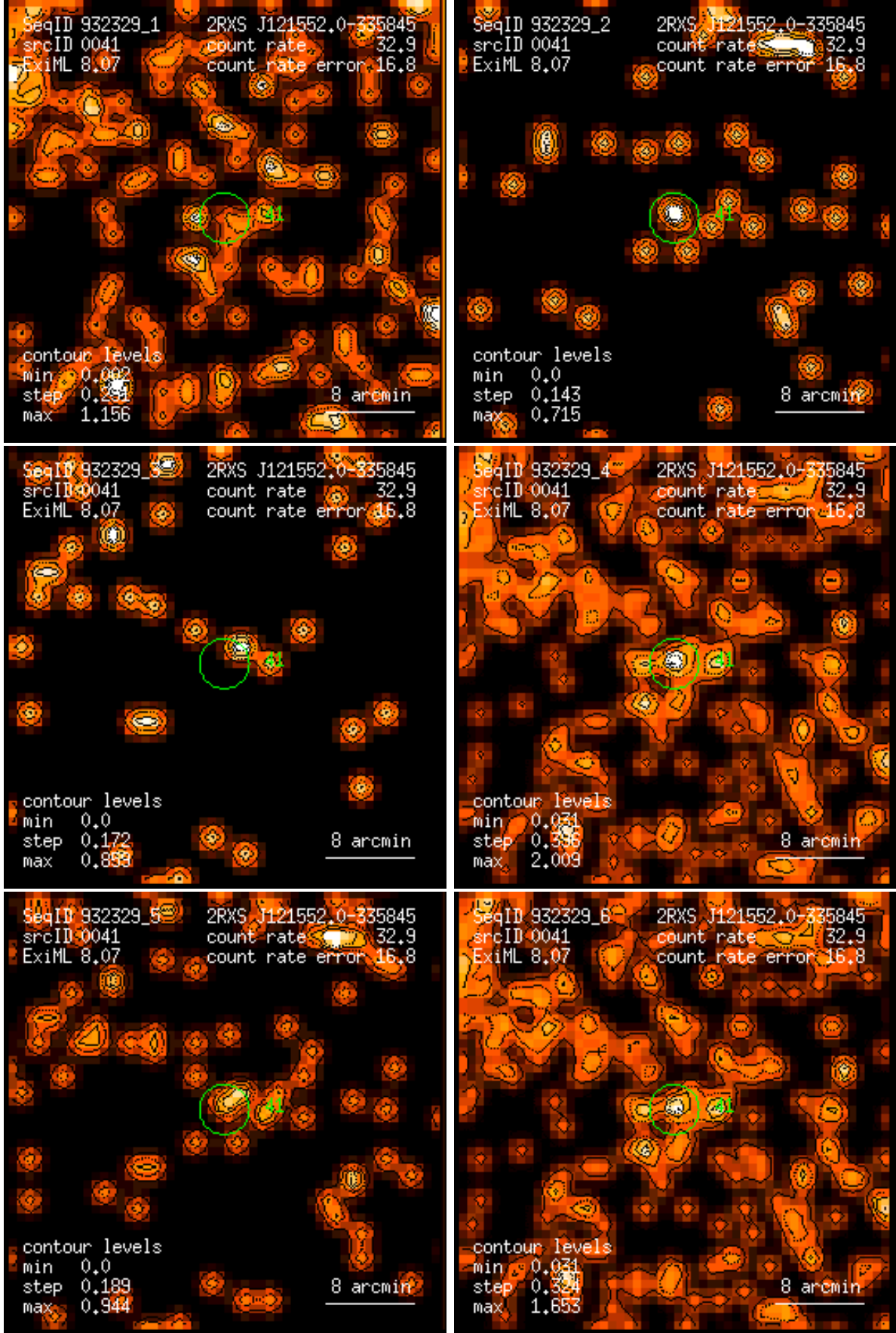
Figure 41: RASS 932329: detection 0041: band rate images, Gaussian filter: (1) PSPC channels 11 – 41, (2) 52 – 90, (3) 91 – 201, (4) 11 – 235, (5) 52 – 201, (6) 11 – 201. Broad band rates in counts/ks. Band rate contour levels in counts/ks/arcmin 2 .
