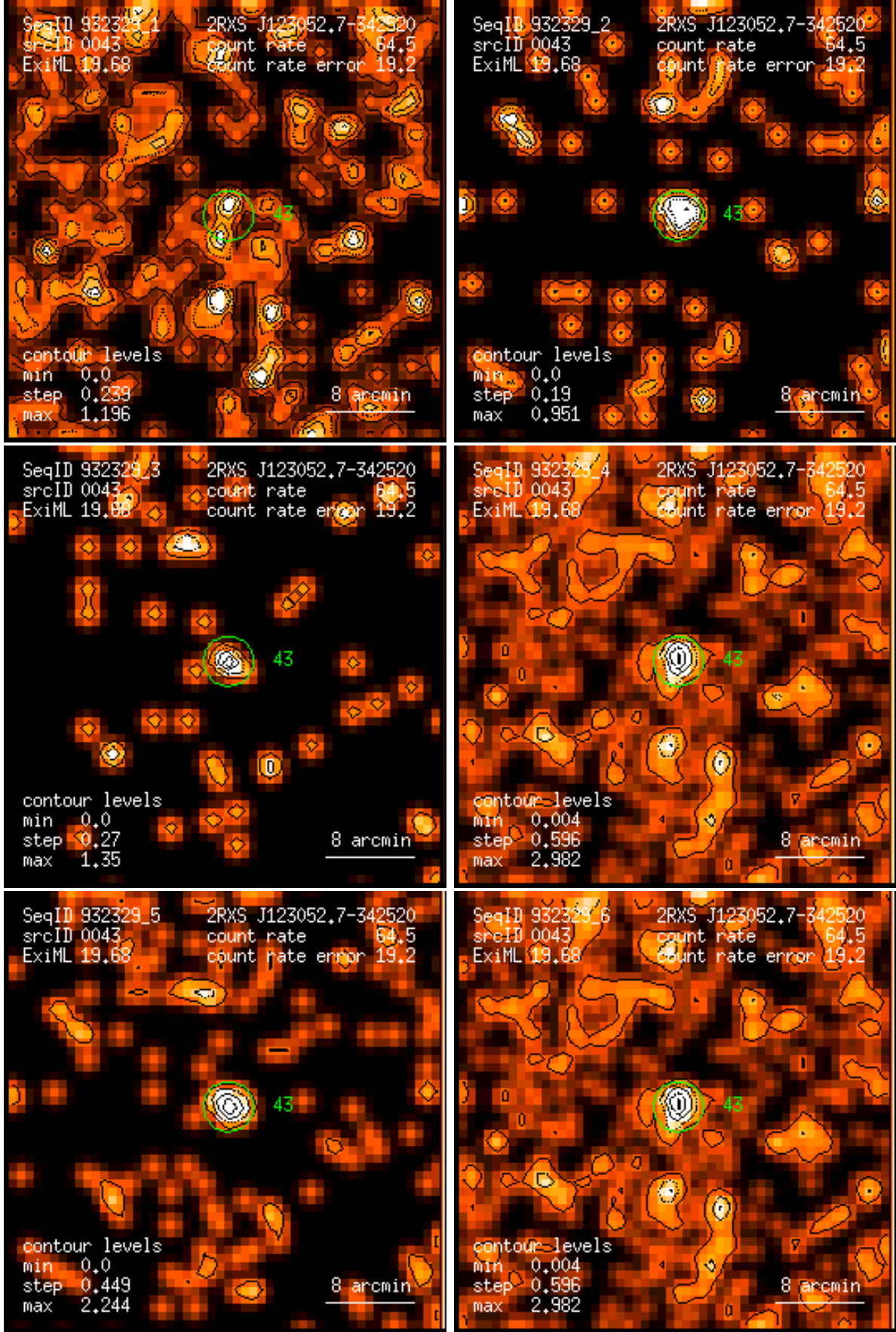
Figure 43: RASS 932329: detection 0043: band rate images, Gaussian filter: (1) PSPC channels 11 – 41, (2) 52 – 90, (3) 91 – 201, (4) 11 – 235, (5) 52 – 201, (6) 11 – 201. Broad band rates in counts/ks. Band rate contour levels in counts/ks/arcmin 2 .
