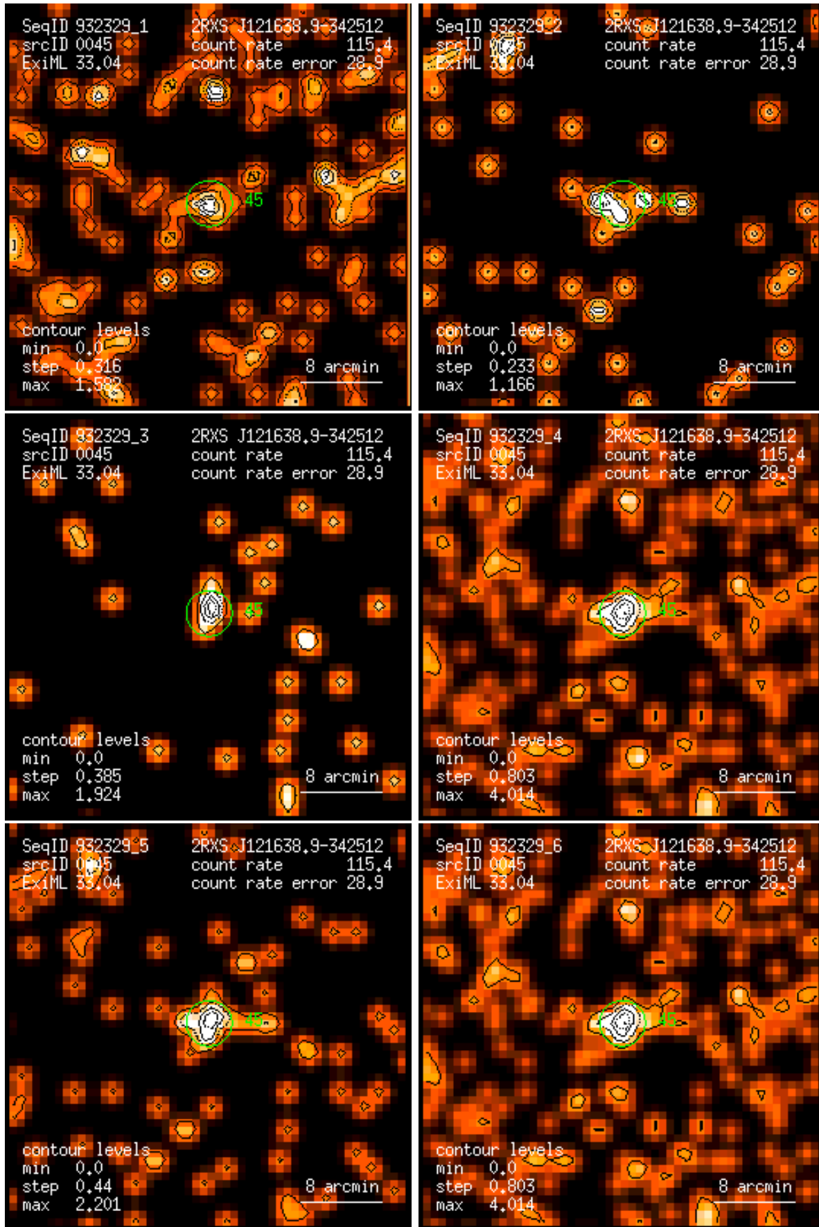
Figure 45: RASS 932329: detection 0045: band rate images, Gaussian filter: (1) PSPC channels 11 – 41, (2) 52 – 90, (3) 91 – 201, (4) 11 – 235, (5) 52 – 201, (6) 11 – 201. Broad band rates in counts/ks. Band rate contour levels in counts/ks/arcmin 2 .
