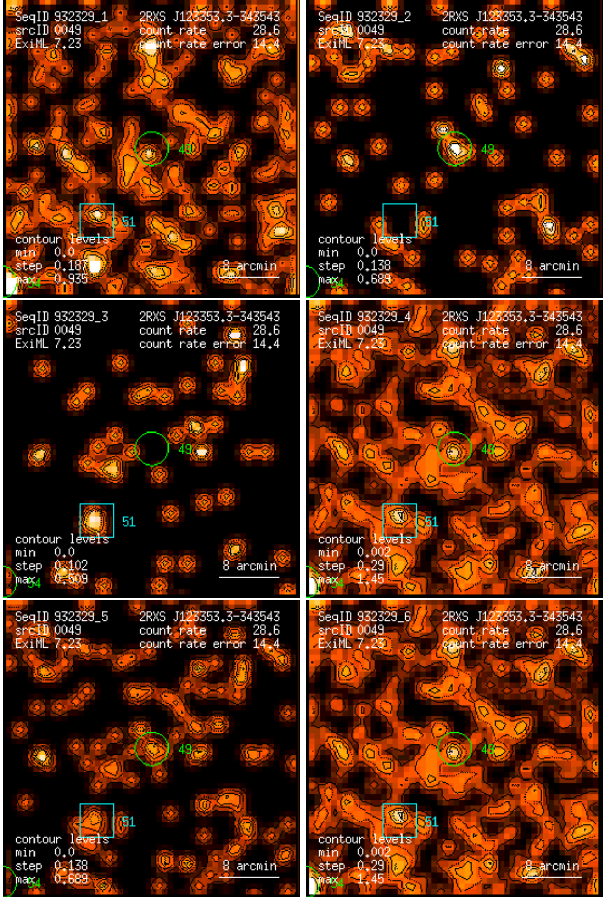
Figure 49: RASS 932329: detection 0049: band rate images, Gaussian filter: (1) PSPC channels 11 – 41, (2) 52 – 90, (3) 91 – 201, (4) 11 – 235, (5) 52 – 201, (6) 11 – 201. Broad band rates in counts/ks. Band rate contour levels in counts/ks/arcmin 2 .
