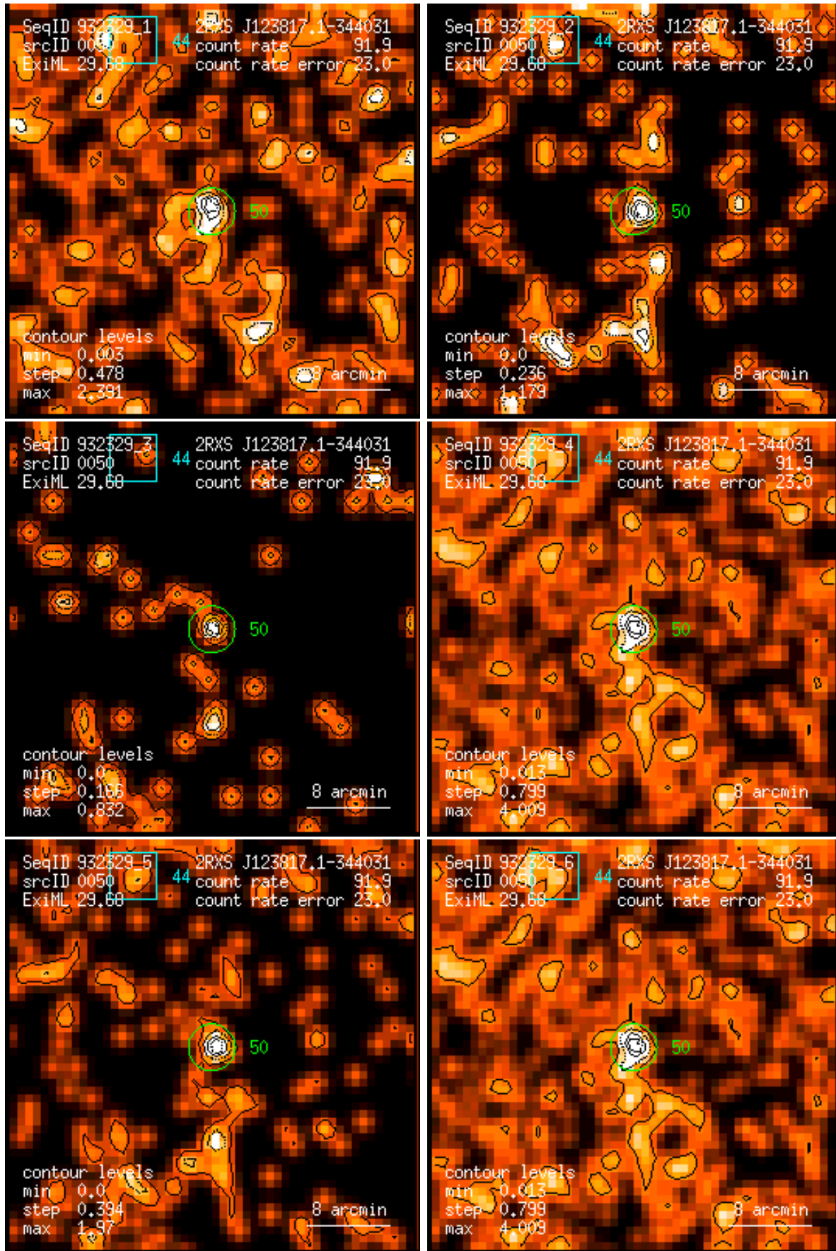
Figure 50: RASS 932329: detection 0050: band rate images, Gaussian filter: (1) PSPC channels 11 – 41, (2) 52 – 90, (3) 91 – 201, (4) 11 – 235, (5) 52 – 201, (6) 11 – 201. Broad band rates in counts/ks. Band rate contour levels in counts/ks/arcmin 2 .
