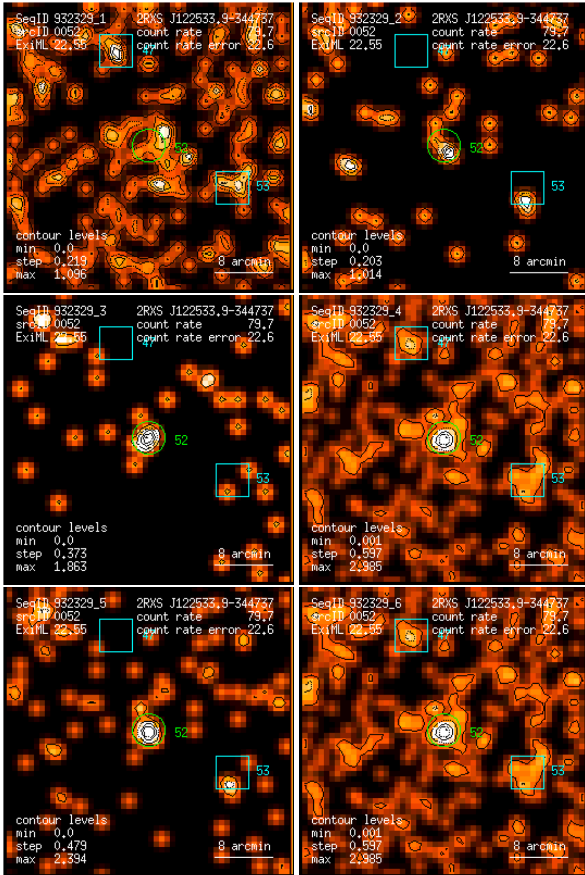
Figure 52: RASS 932329: detection 0052: band rate images, Gaussian filter: (1) PSPC channels 11 – 41, (2) 52 – 90, (3) 91 – 201, (4) 11 – 235, (5) 52 – 201, (6) 11 – 201. Broad band rates in counts/ks. Band rate contour levels in counts/ks/arcmin 2 .
