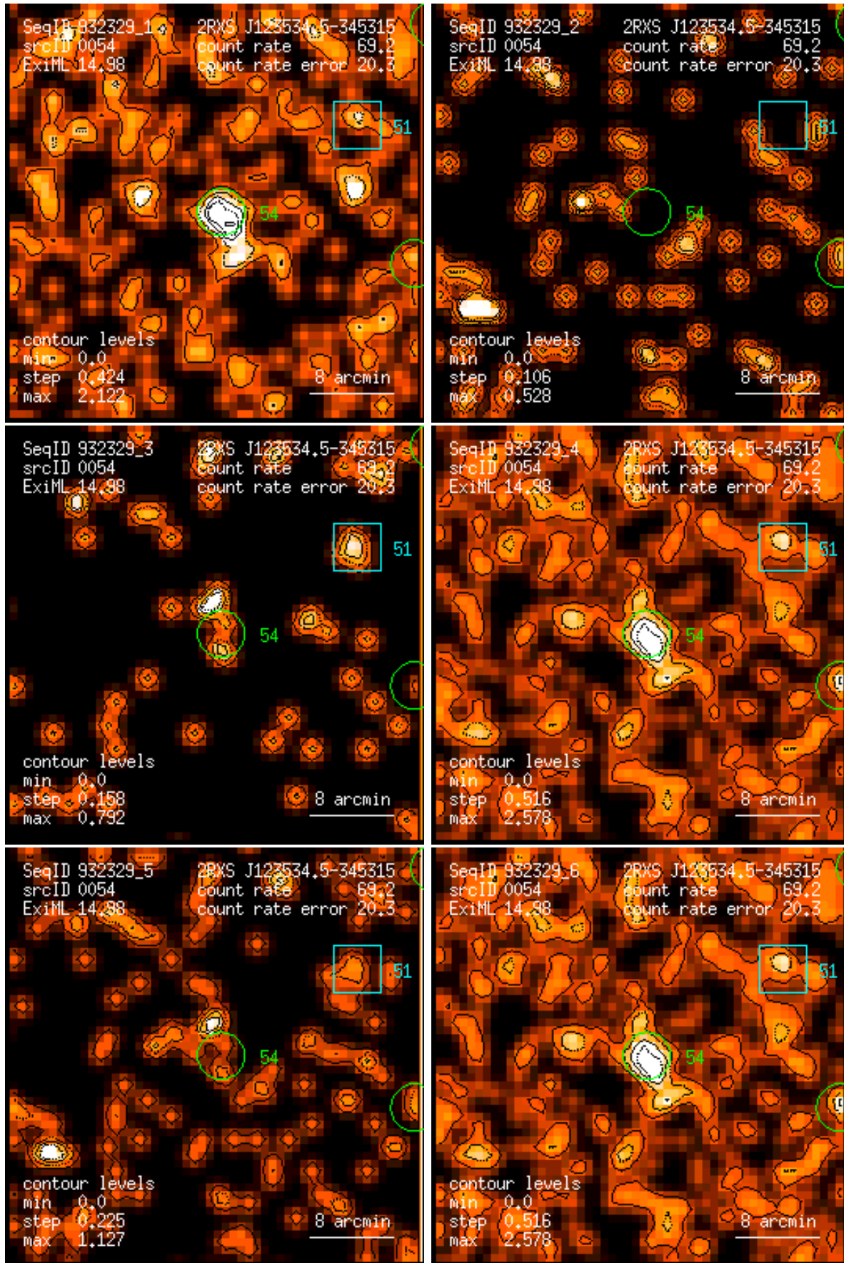
Figure 54: RASS 932329: detection 0054: band rate images, Gaussian filter: (1) PSPC channels 11 – 41, (2) 52 – 90, (3) 91 – 201, (4) 11 – 235, (5) 52 – 201, (6) 11 – 201. Broad band rates in counts/ks. Band rate contour levels in counts/ks/arcmin 2 .
