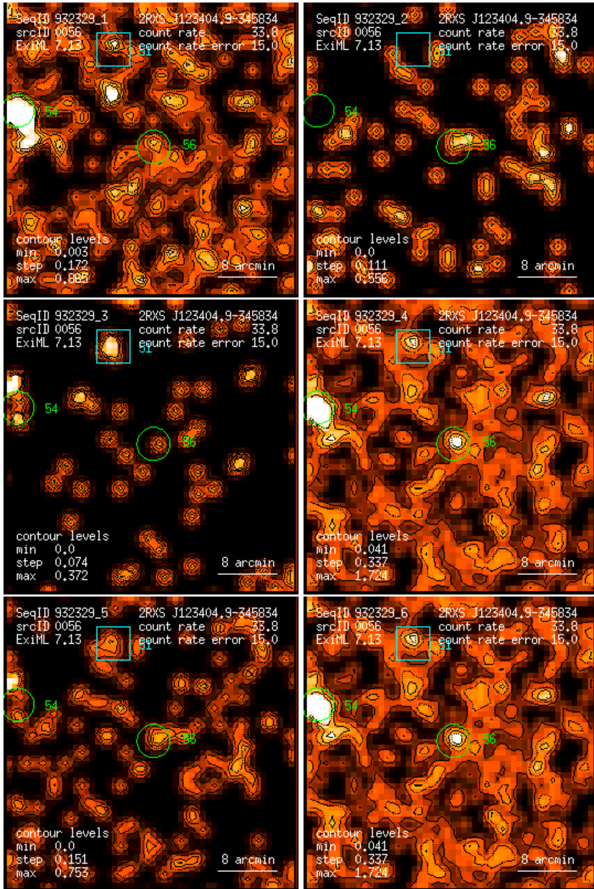
Figure 56: RASS 932329: detection 0056: band rate images, Gaussian filter: (1) PSPC channels 11 – 41, (2) 52 – 90, (3) 91 – 201, (4) 11 – 235, (5) 52 – 201, (6) 11 – 201. Broad band rates in counts/ks. Band rate contour levels in counts/ks/arcmin 2 .
