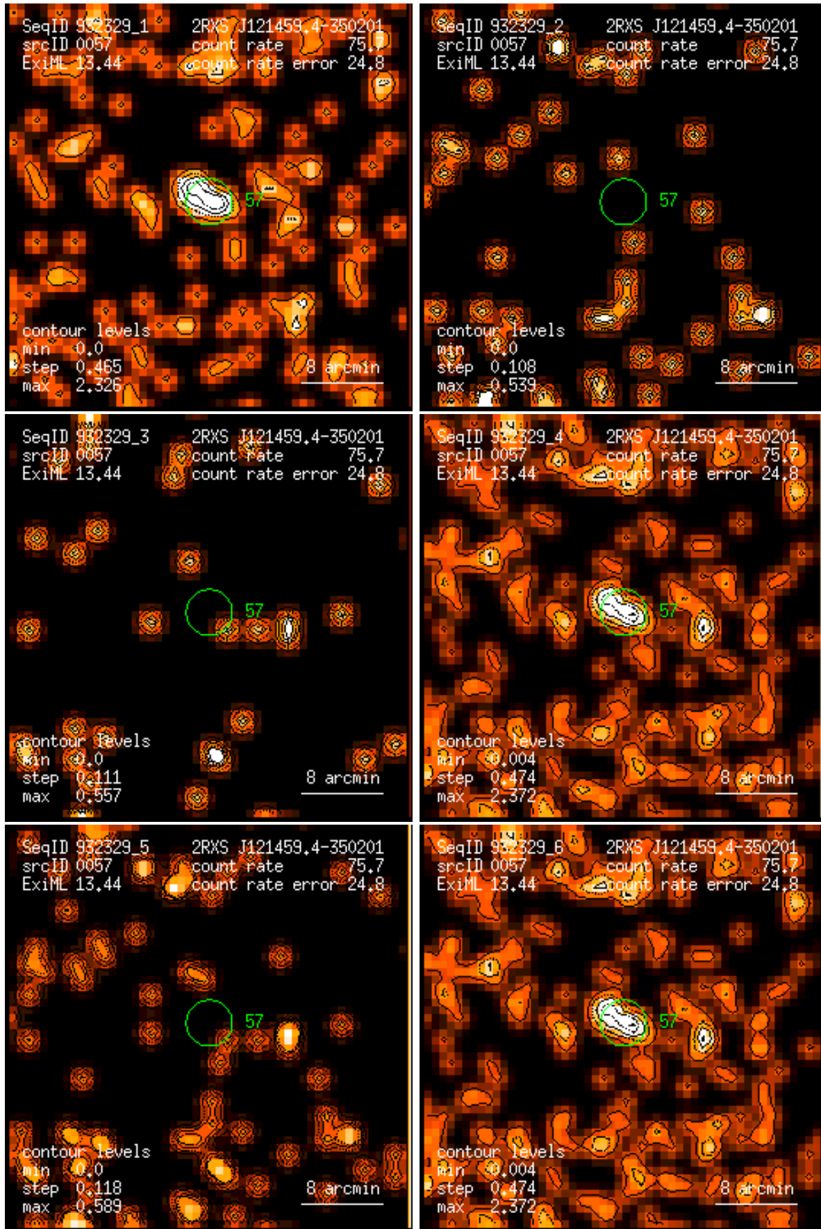
Figure 57: RASS 932329: detection 0057: band rate images, Gaussian filter: (1) PSPC channels 11 – 41, (2) 52 – 90, (3) 91 – 201, (4) 11 – 235, (5) 52 – 201, (6) 11 – 201. Broad band rates in counts/ks. Band rate contour levels in counts/ks/arcmin 2 .
