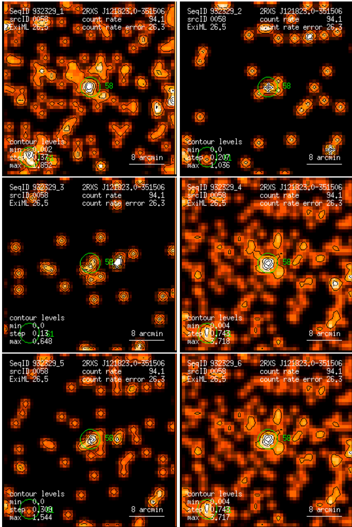
Figure 58: RASS 932329: detection 0058: band rate images, Gaussian filter: (1) PSPC channels 11 – 41, (2) 52 – 90, (3) 91 – 201, (4) 11 – 235, (5) 52 – 201, (6) 11 – 201. Broad band rates in counts/ks. Band rate contour levels in counts/ks/arcmin 2 .
