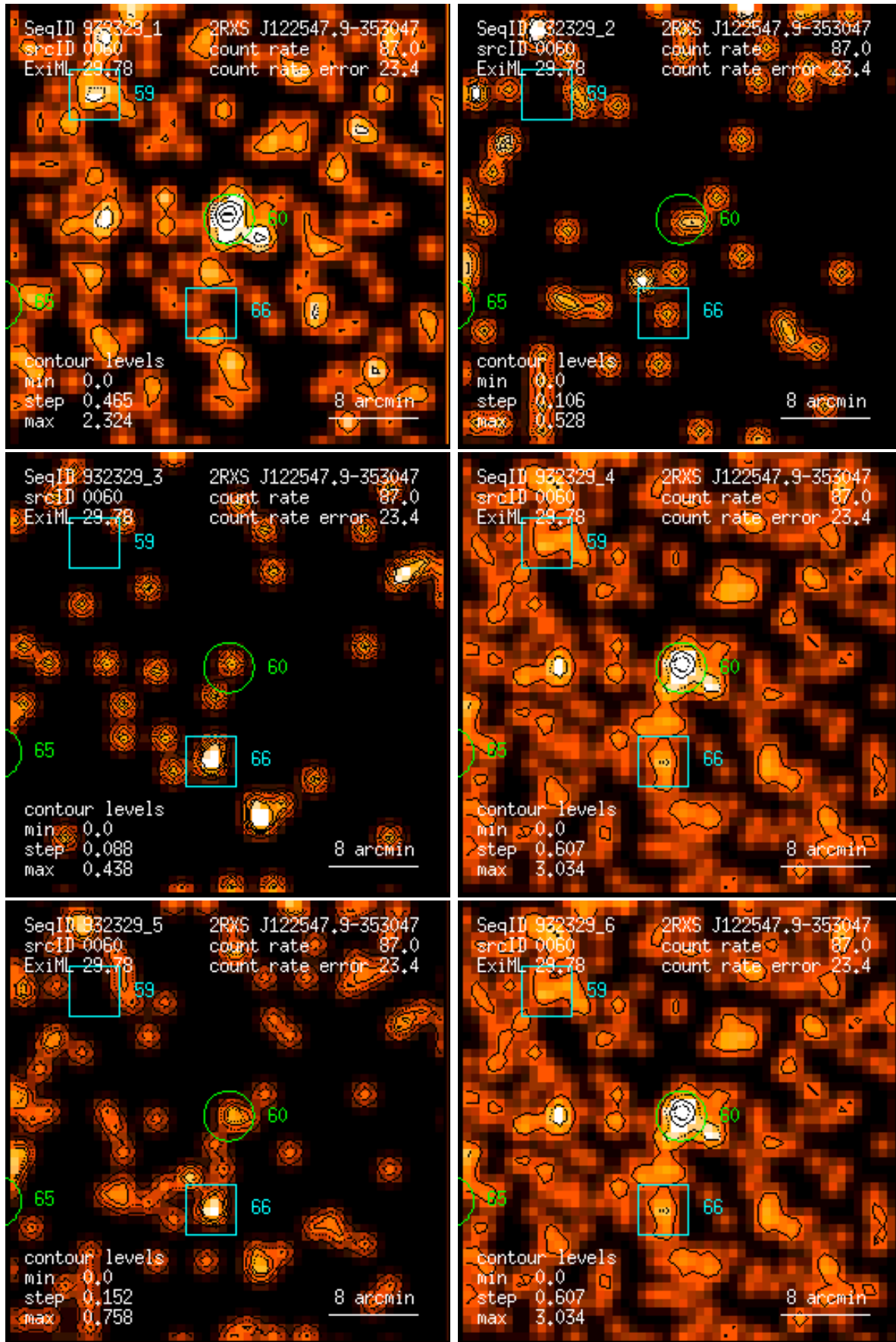
Figure 60: RASS 932329: detection 0060: band rate images, Gaussian filter: (1) PSPC channels 11 – 41, (2) 52 – 90, (3) 91 – 201, (4) 11 – 235, (5) 52 – 201, (6) 11 – 201. Broad band rates in counts/ks. Band rate contour levels in counts/ks/arcmin 2 .
