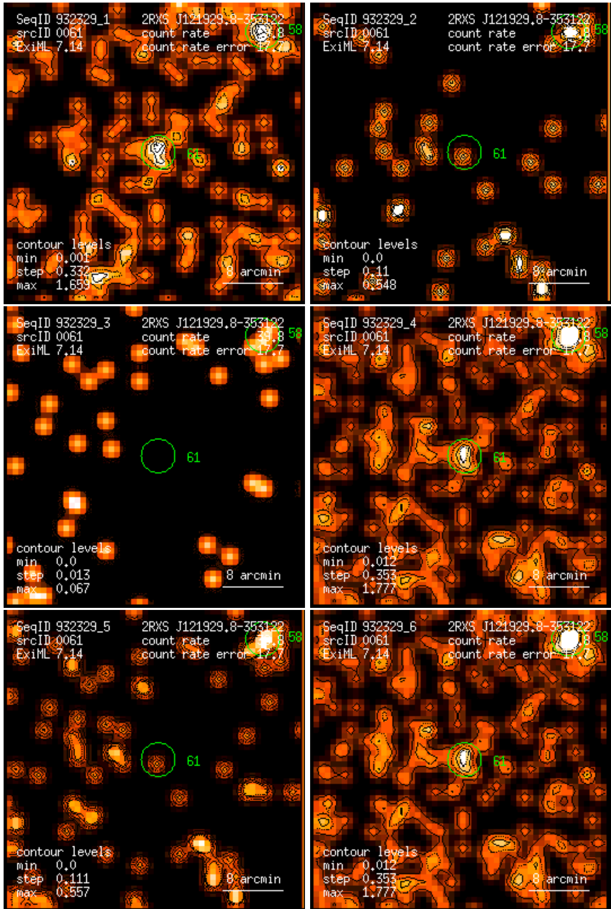
Figure 61: RASS 932329: detection 0061: band rate images, Gaussian filter: (1) PSPC channels 11 – 41, (2) 52 – 90, (3) 91 – 201, (4) 11 – 235, (5) 52 – 201, (6) 11 – 201. Broad band rates in counts/ks. Band rate contour levels in counts/ks/arcmin 2 .
