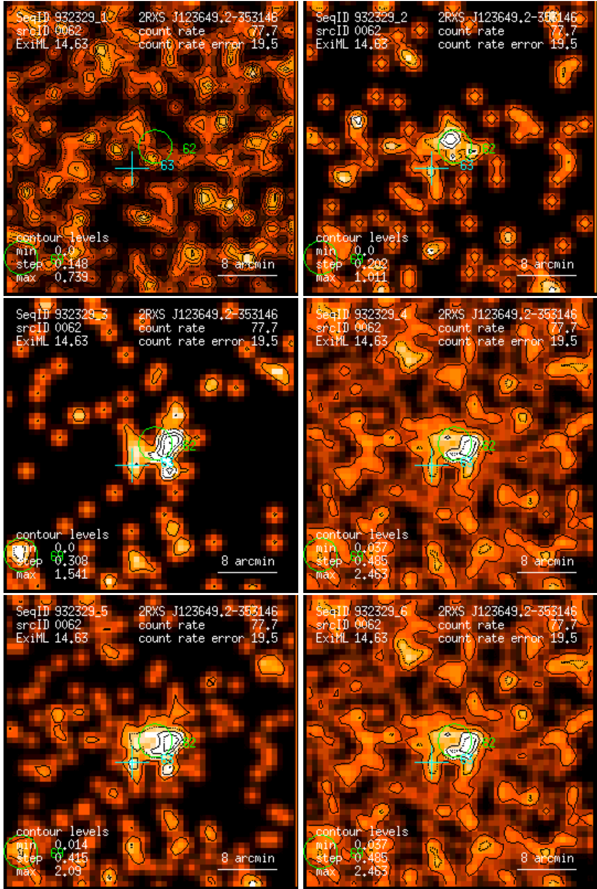
Figure 62: RASS 932329: detection 0062: band rate images, Gaussian filter: (1) PSPC channels 11 – 41, (2) 52 – 90, (3) 91 – 201, (4) 11 – 235, (5) 52 – 201, (6) 11 – 201. Broad band rates in counts/ks. Band rate contour levels in counts/ks/arcmin 2 .
