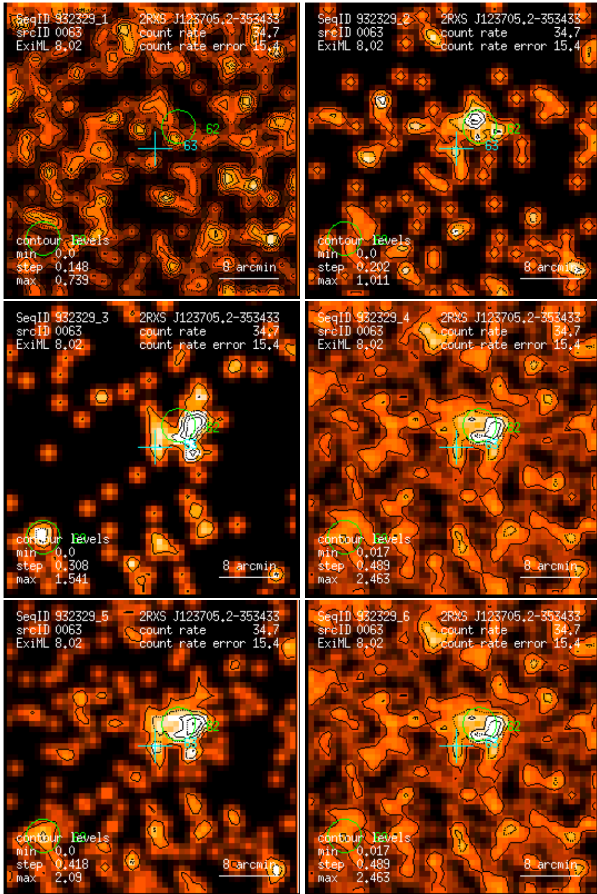
Figure 63: RASS 932329: detection 0063: band rate images, Gaussian filter: (1) PSPC channels 11 – 41, (2) 52 – 90, (3) 91 – 201, (4) 11 – 235, (5) 52 – 201, (6) 11 – 201. Broad band rates in counts/ks. Band rate contour levels in counts/ks/arcmin 2 .
