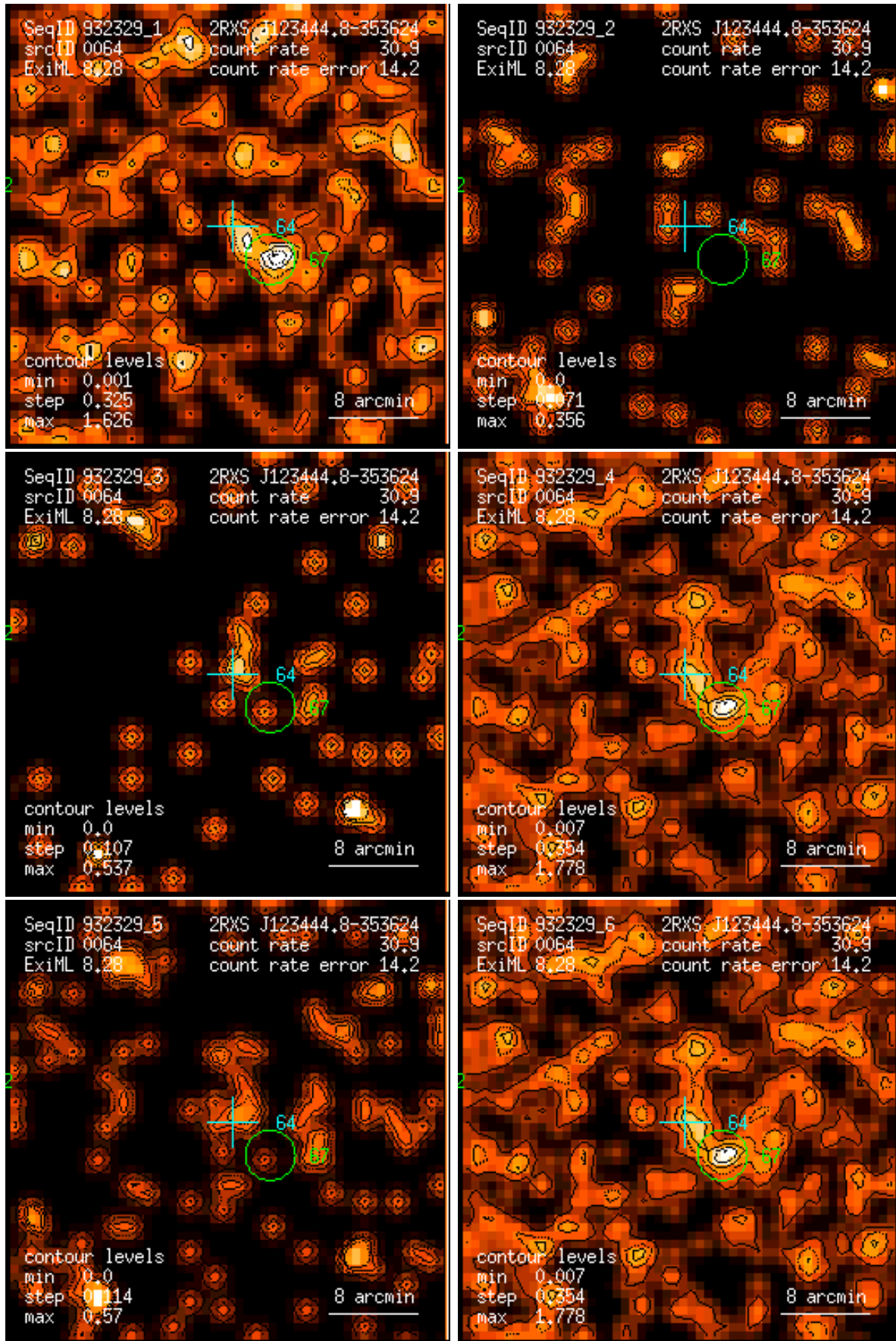
Figure 64: RASS 932329: detection 0064: band rate images, Gaussian filter: (1) PSPC channels 11 – 41, (2) 52 – 90, (3) 91 – 201, (4) 11 – 235, (5) 52 – 201, (6) 11 – 201. Broad band rates in counts/ks. Band rate contour levels in counts/ks/arcmin 2 .
