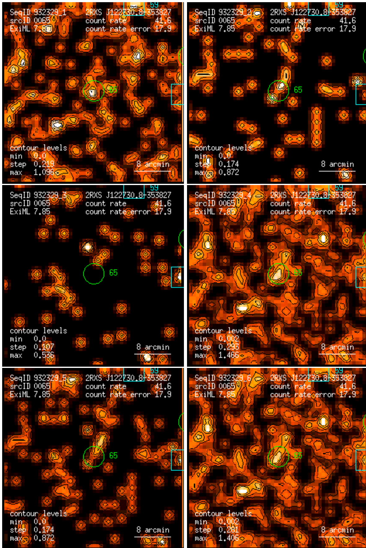
Figure 65: RASS 932329: detection 0065: band rate images, Gaussian filter: (1) PSPC channels 11 – 41, (2) 52 – 90, (3) 91 – 201, (4) 11 – 235, (5) 52 – 201, (6) 11 – 201. Broad band rates in counts/ks. Band rate contour levels in counts/ks/arcmin 2 .
