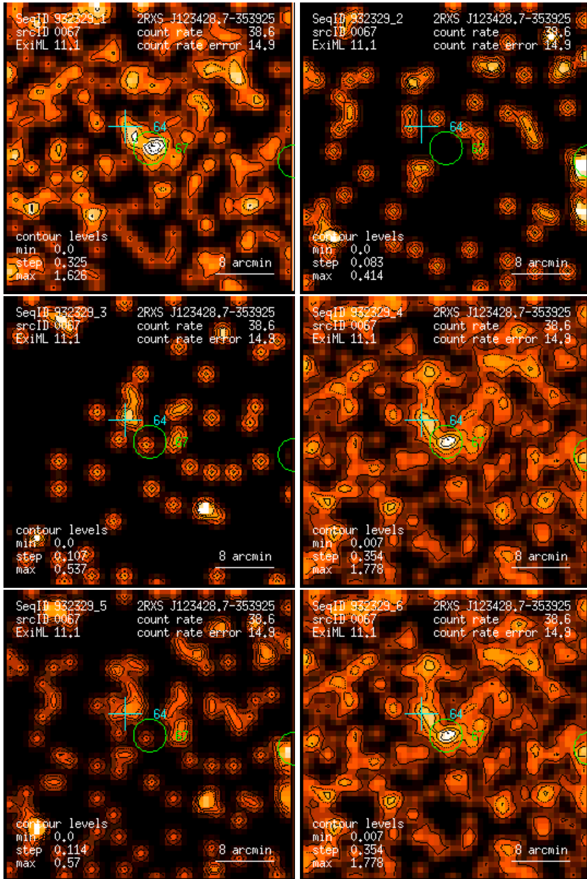
Figure 67: RASS 932329: detection 0067: band rate images, Gaussian filter: (1) PSPC channels 11 – 41, (2) 52 – 90, (3) 91 – 201, (4) 11 – 235, (5) 52 – 201, (6) 11 – 201. Broad band rates in counts/ks. Band rate contour levels in counts/ks/arcmin 2 .
