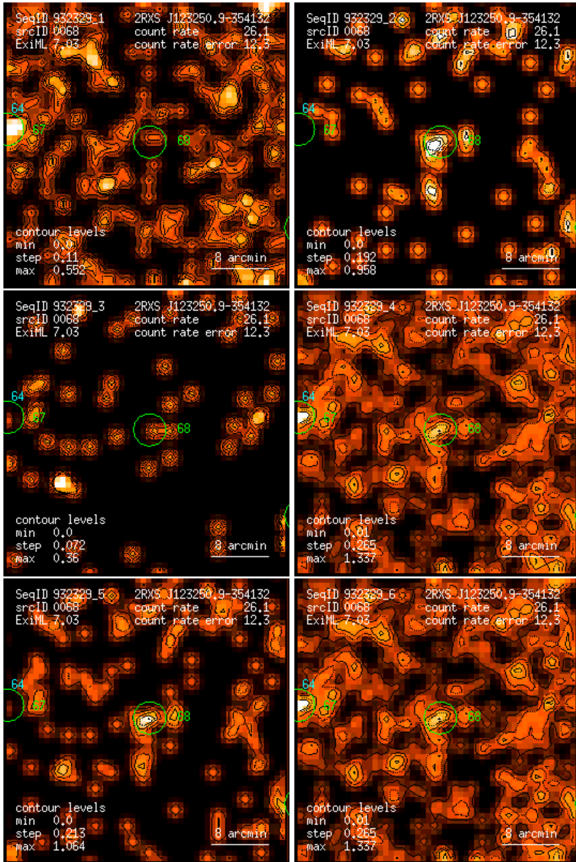
Figure 68: RASS 932329: detection 0068: band rate images, Gaussian filter: (1) PSPC channels 11 – 41, (2) 52 – 90, (3) 91 – 201, (4) 11 – 235, (5) 52 – 201, (6) 11 – 201. Broad band rates in counts/ks. Band rate contour levels in counts/ks/arcmin 2 .
