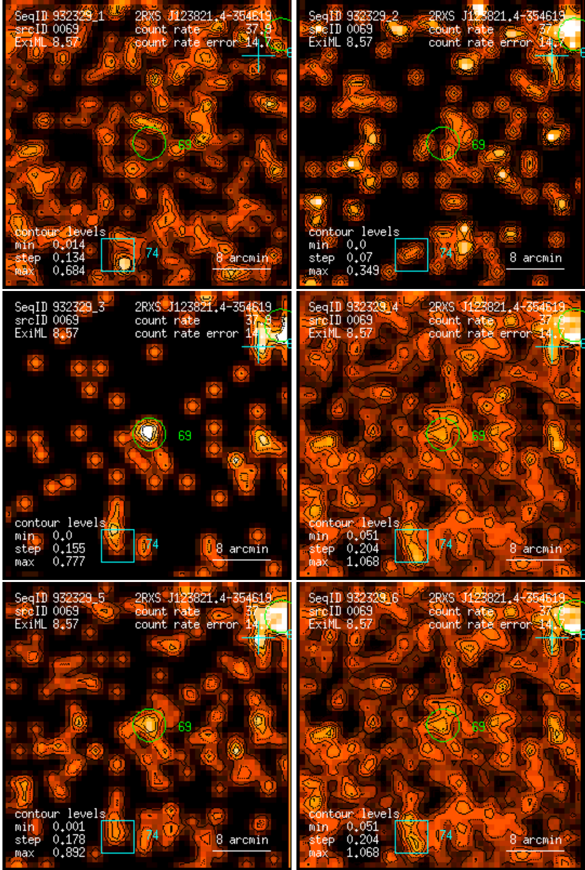
Figure 69: RASS 932329: detection 0069: band rate images, Gaussian filter: (1) PSPC channels 11 – 41, (2) 52 – 90, (3) 91 – 201, (4) 11 – 235, (5) 52 – 201, (6) 11 – 201. Broad band rates in counts/ks. Band rate contour levels in counts/ks/arcmin 2 .
