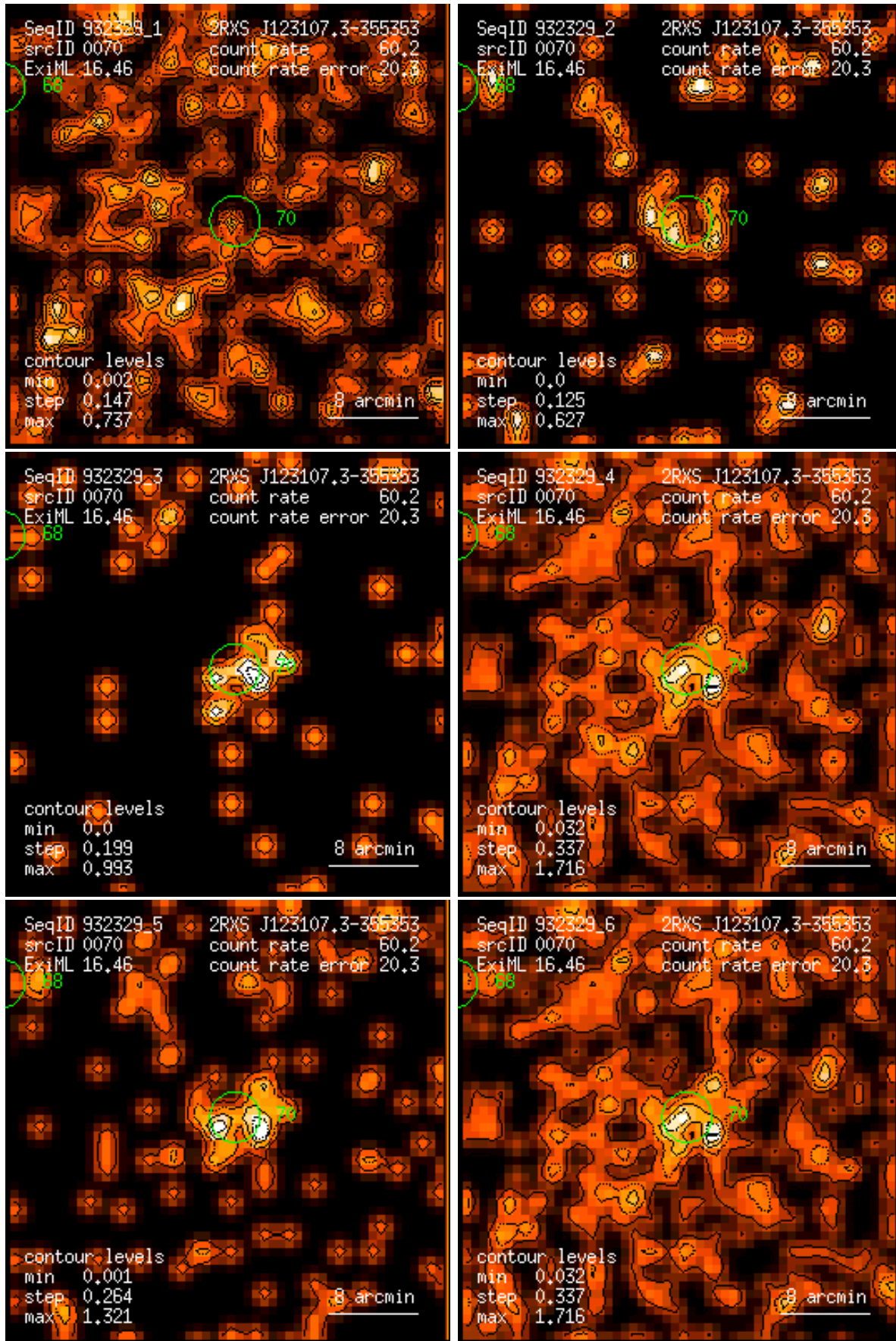
Figure 70: RASS 932329: detection 0070: band rate images, Gaussian filter: (1) PSPC channels 11 – 41, (2) 52 – 90, (3) 91 – 201, (4) 11 – 235, (5) 52 – 201, (6) 11 – 201. Broad band rates in counts/ks. Band rate contour levels in counts/ks/arcmin 2 .
