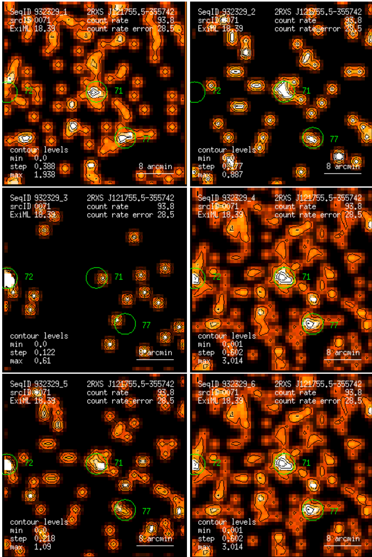
Figure 71: RASS 932329: detection 0071: band rate images, Gaussian filter: (1) PSPC channels 11 – 41, (2) 52 – 90, (3) 91 – 201, (4) 11 – 235, (5) 52 – 201, (6) 11 – 201. Broad band rates in counts/ks. Band rate contour levels in counts/ks/arcmin 2 .
