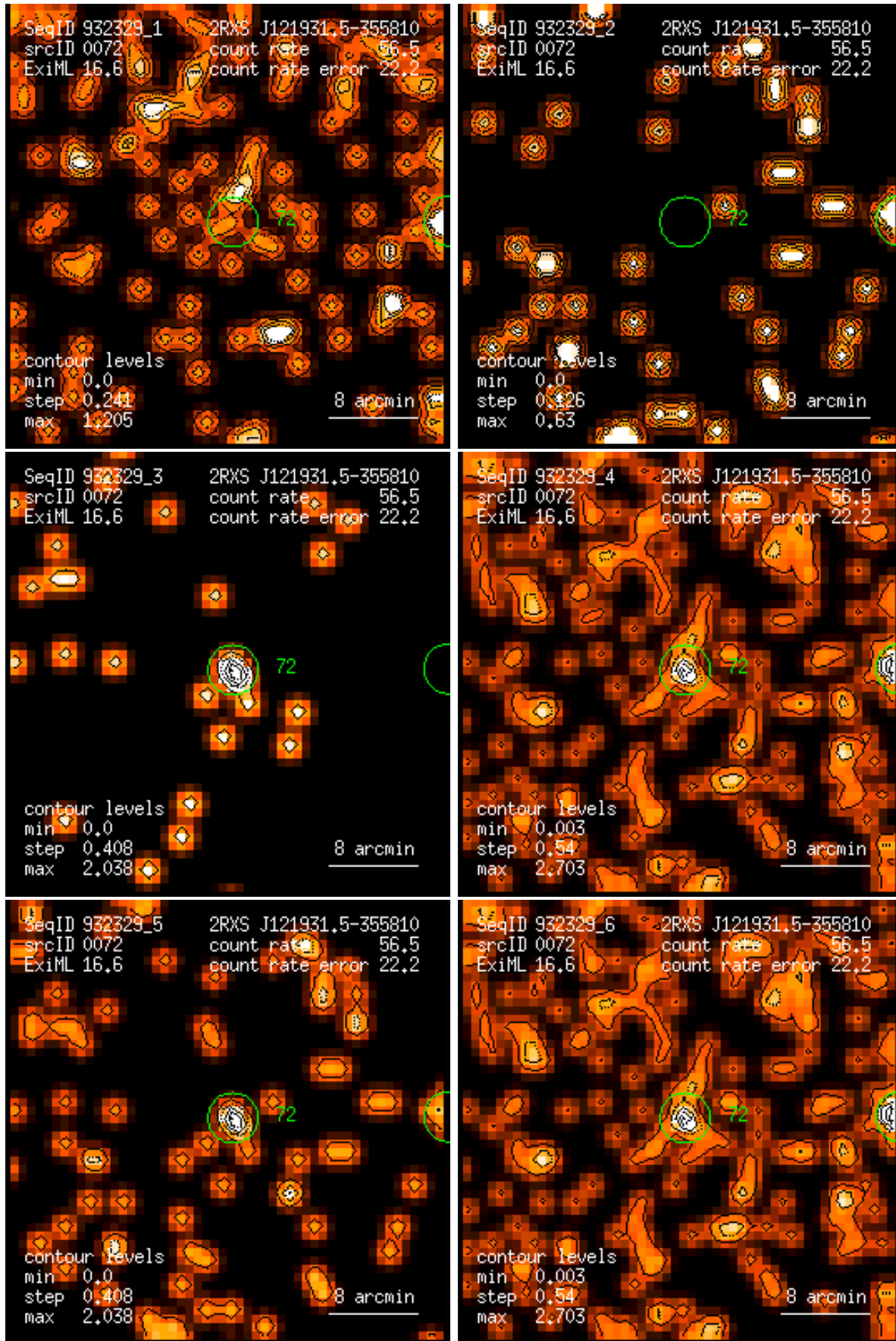
Figure 72: RASS 932329: detection 0072: band rate images, Gaussian filter: (1) PSPC channels 11 – 41, (2) 52 – 90, (3) 91 – 201, (4) 11 – 235, (5) 52 – 201, (6) 11 – 201. Broad band rates in counts/ks. Band rate contour levels in counts/ks/arcmin 2 .
