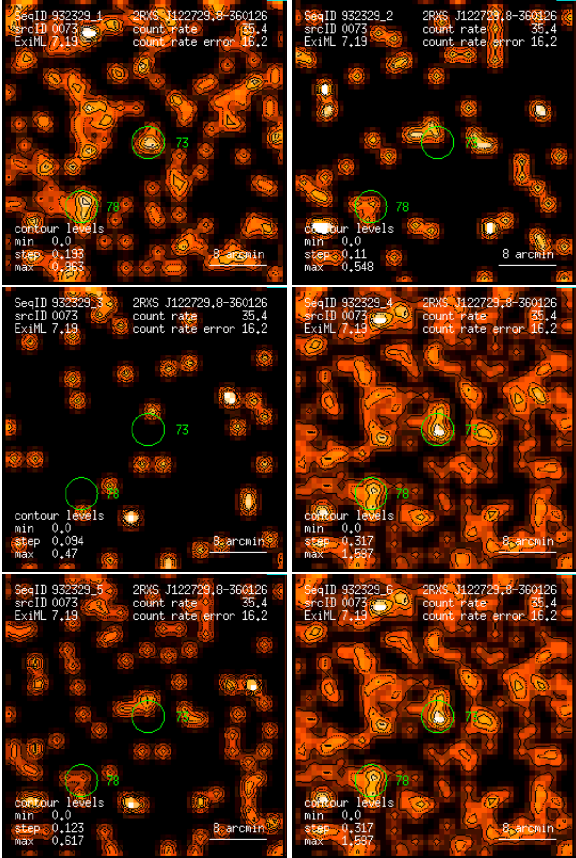
Figure 73: RASS 932329: detection 0073: band rate images, Gaussian filter: (1) PSPC channels 11 – 41, (2) 52 – 90, (3) 91 – 201, (4) 11 – 235, (5) 52 – 201, (6) 11 – 201. Broad band rates in counts/ks. Band rate contour levels in counts/ks/arcmin 2 .
