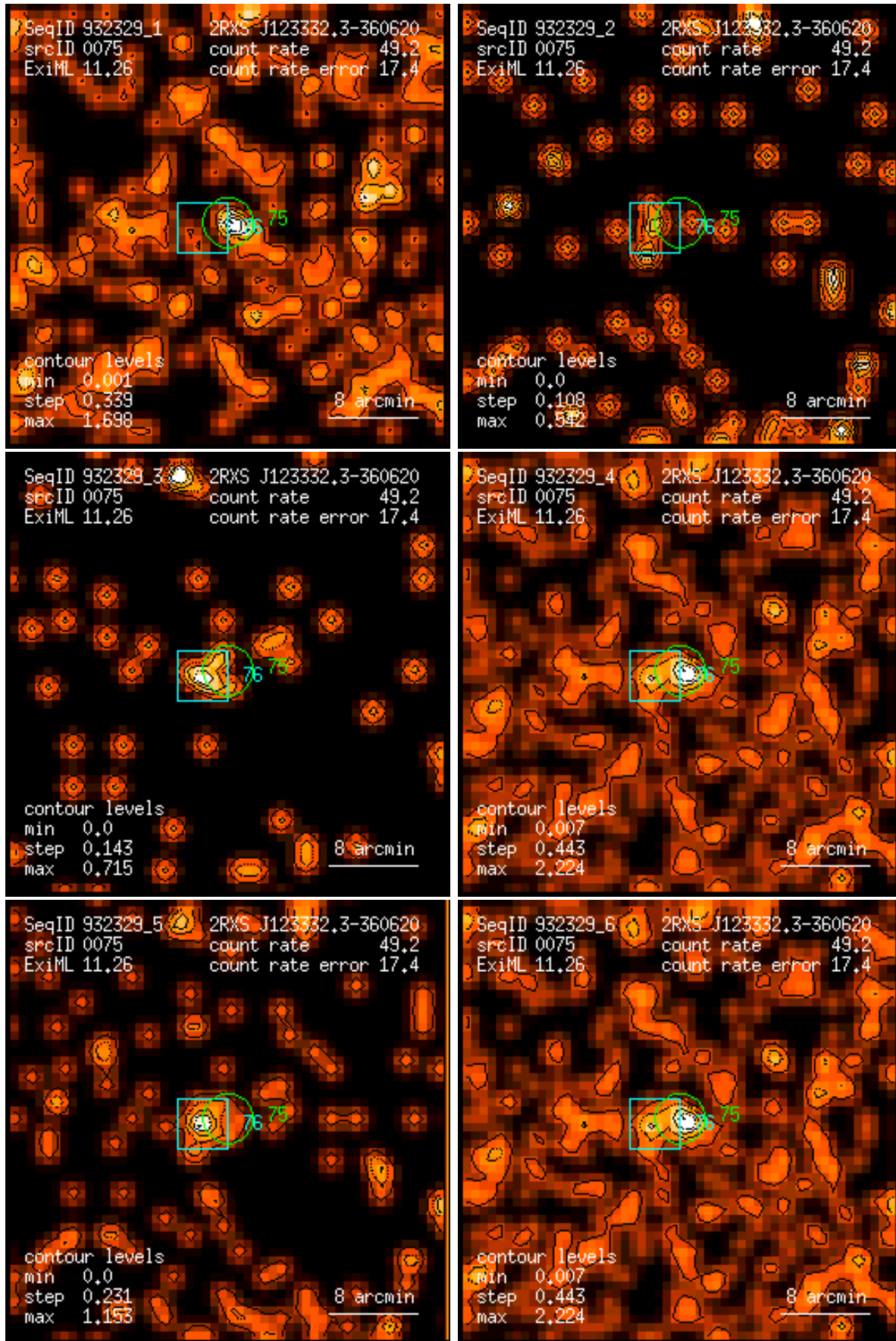
Figure 75: RASS 932329: detection 0075: band rate images, Gaussian filter: (1) PSPC channels 11 – 41, (2) 52 – 90, (3) 91 – 201, (4) 11 – 235, (5) 52 – 201, (6) 11 – 201. Broad band rates in counts/ks. Band rate contour levels in counts/ks/arcmin 2 .
