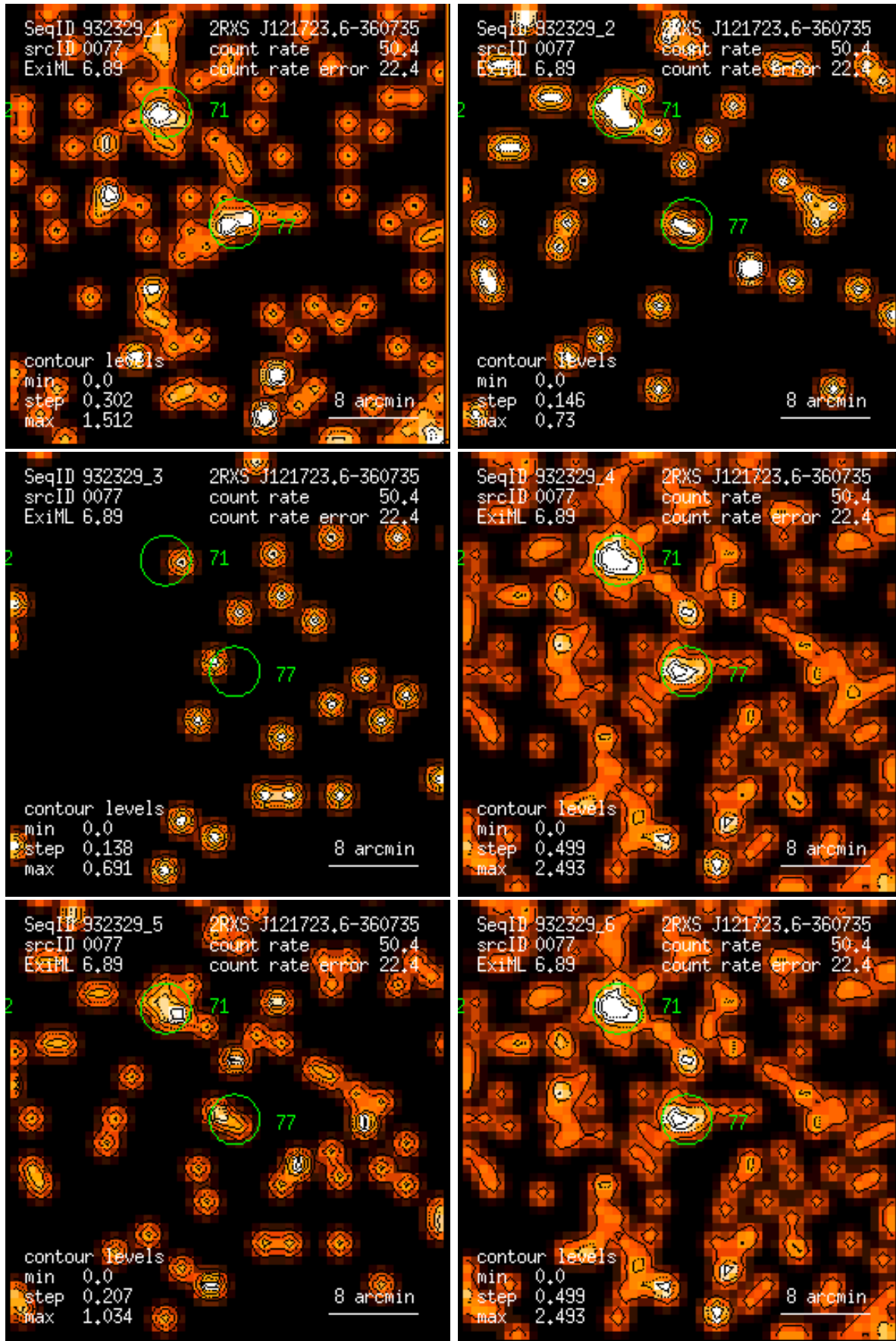
Figure 77: RASS 932329: detection 0077: band rate images, Gaussian filter: (1) PSPC channels 11 – 41, (2) 52 – 90, (3) 91 – 201, (4) 11 – 235, (5) 52 – 201, (6) 11 – 201. Broad band rates in counts/ks. Band rate contour levels in counts/ks/arcmin 2 .
