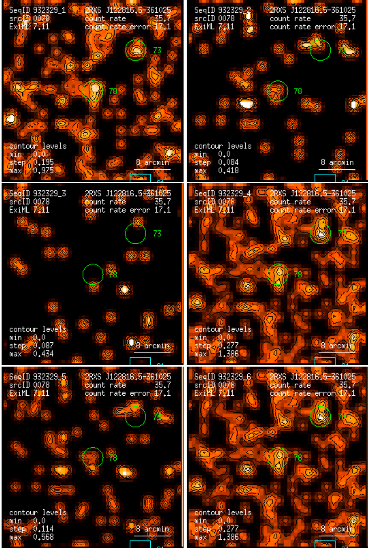
Figure 78: RASS 932329: detection 0078: band rate images, Gaussian filter: (1) PSPC channels 11 – 41, (2) 52 – 90, (3) 91 – 201, (4) 11 – 235, (5) 52 – 201, (6) 11 – 201. Broad band rates in counts/ks. Band rate contour levels in counts/ks/arcmin 2 .
