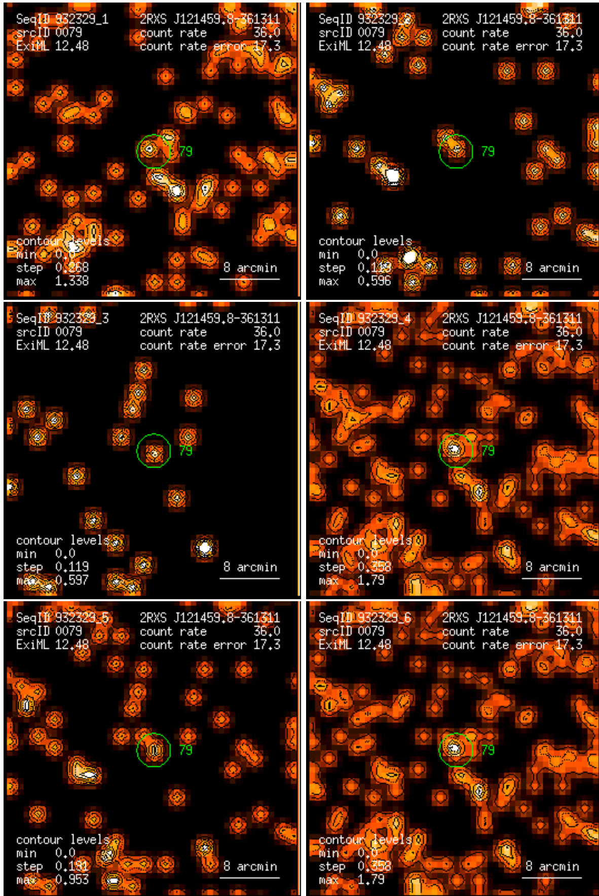
Figure 79: RASS 932329: detection 0079: band rate images, Gaussian filter: (1) PSPC channels 11 – 41, (2) 52 – 90, (3) 91 – 201, (4) 11 – 235, (5) 52 – 201, (6) 11 – 201. Broad band rates in counts/ks. Band rate contour levels in counts/ks/arcmin 2 .
