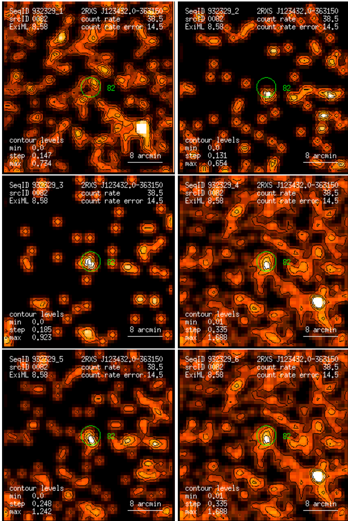
Figure 82: RASS 932329: detection 0082: band rate images, Gaussian filter: (1) PSPC channels 11 – 41, (2) 52 – 90, (3) 91 – 201, (4) 11 – 235, (5) 52 – 201, (6) 11 – 201. Broad band rates in counts/ks. Band rate contour levels in counts/ks/arcmin 2 .
