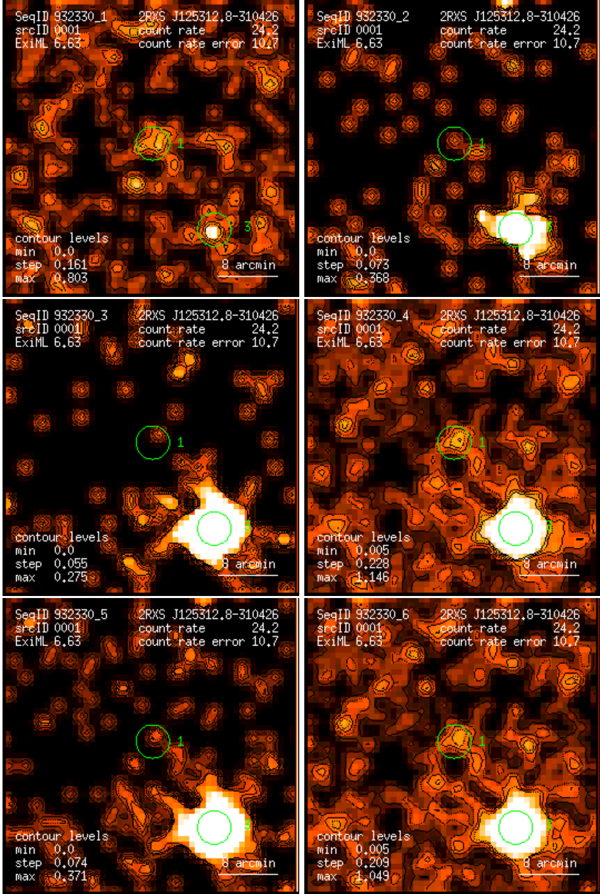
Figure 1: RASS 932330: detection 0001: band rate images, Gaussian filter: (1) PSPC channels 11 – 41, (2) 52 – 90, (3) 91 – 201, (4) 11 – 235, (5) 52 – 201, (6) 11 – 201. Broad band rates in counts/ks. Band rate contour levels in counts/ks/arcmin 2 .
