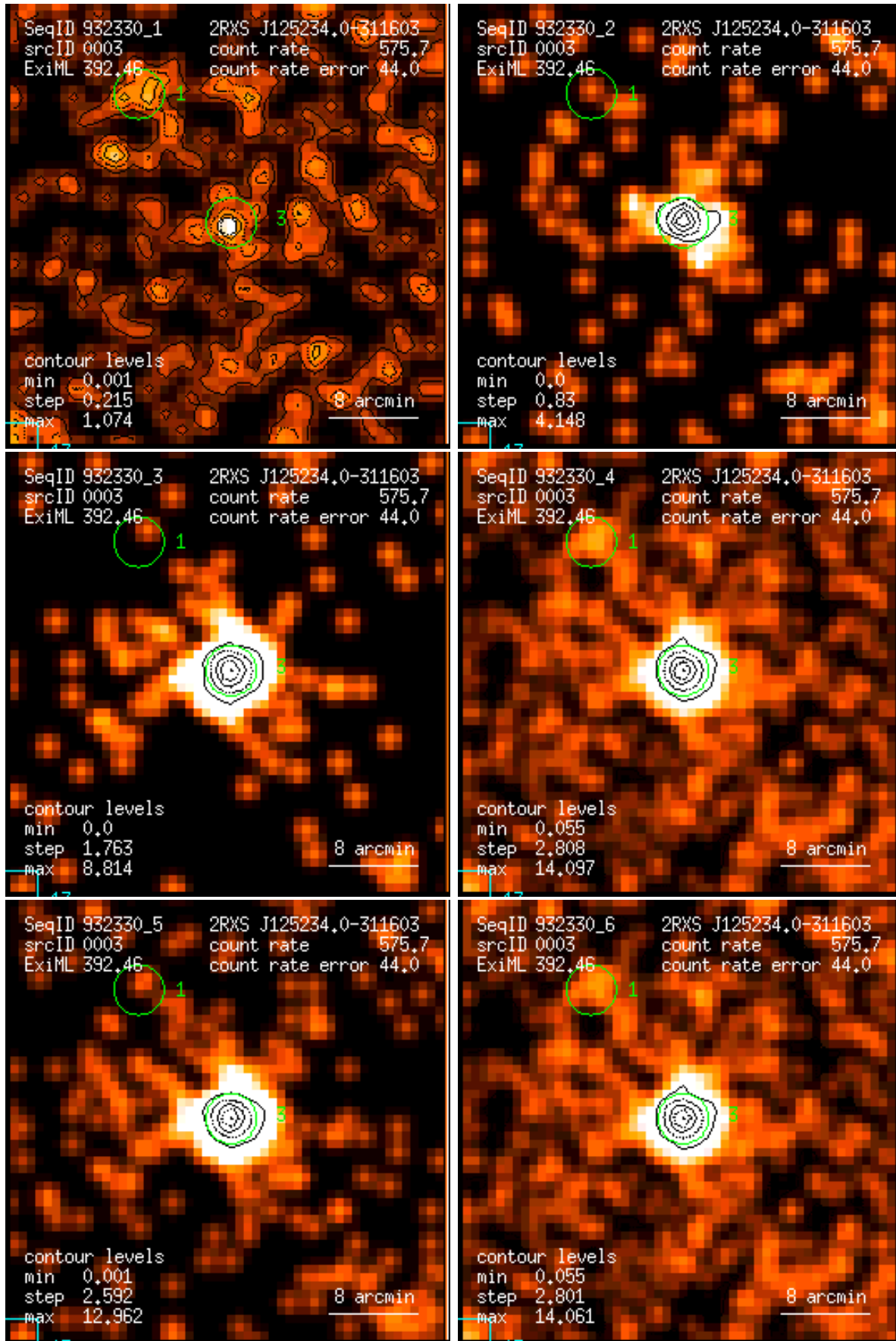
Figure 3: RASS 932330: detection 0003: band rate images, Gaussian filter: (1) PSPC channels 11 – 41, (2) 52 – 90, (3) 91 – 201, (4) 11 – 235, (5) 52 – 201, (6) 11 – 201. Broad band rates in counts/ks. Band rate contour levels in counts/ks/arcmin 2 .
