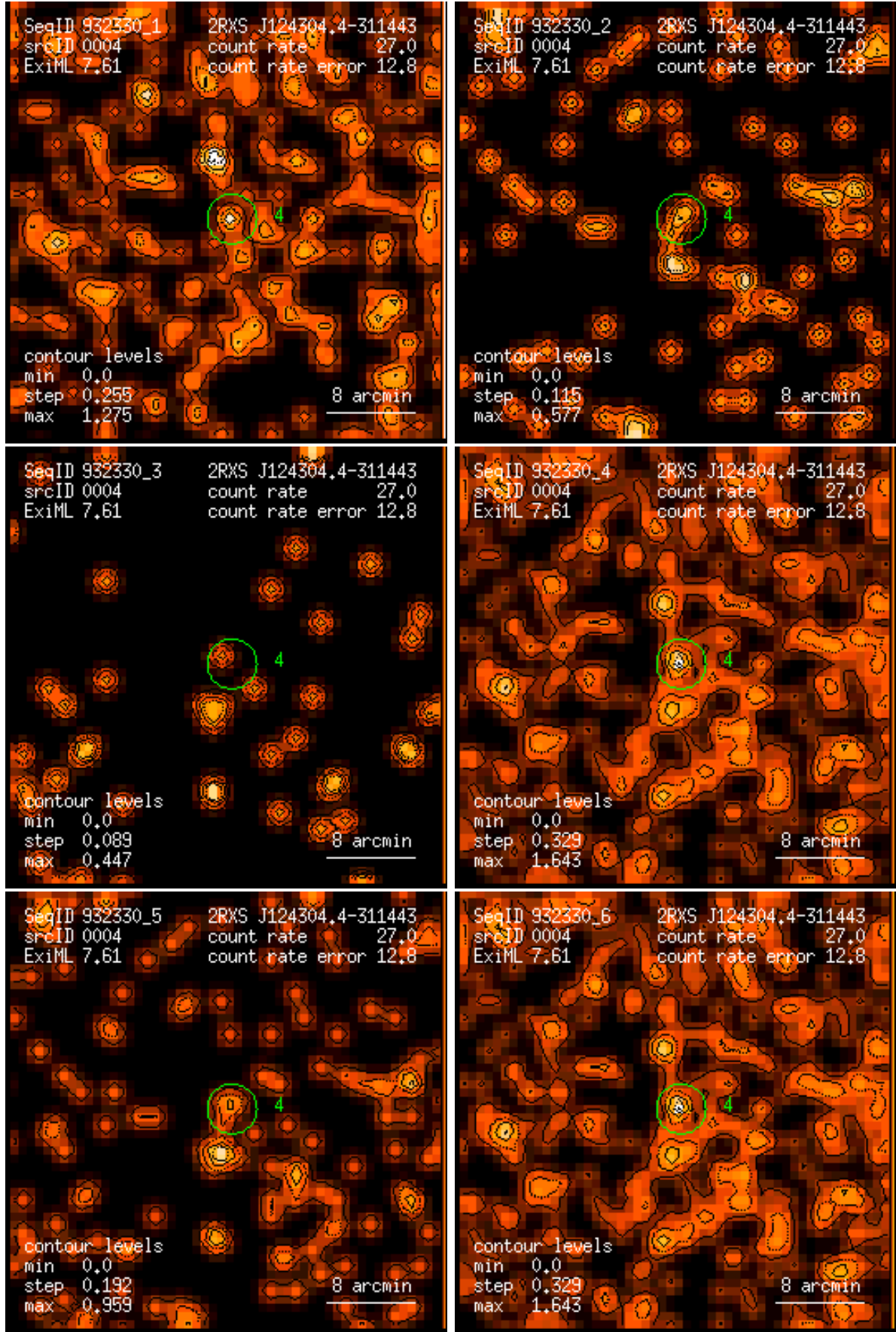
Figure 4: RASS 932330: detection 0004: band rate images, Gaussian filter: (1) PSPC channels 11 – 41, (2) 52 – 90, (3) 91 – 201, (4) 11 – 235, (5) 52 – 201, (6) 11 – 201. Broad band rates in counts/ks. Band rate contour levels in counts/ks/arcmin 2 .
