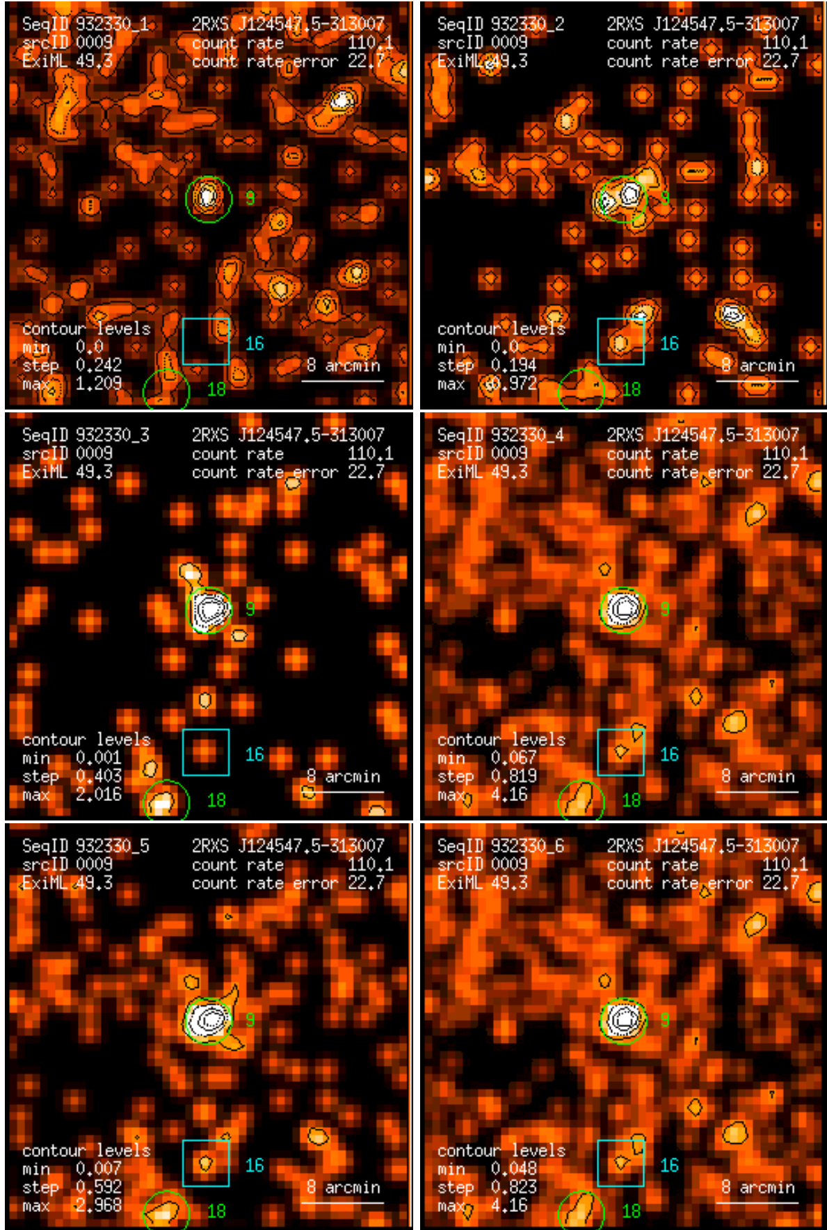
Figure 9: RASS 932330: detection 0009: band rate images, Gaussian filter: (1) PSPC channels 11 – 41, (2) 52 – 90, (3) 91 – 201, (4) 11 – 235, (5) 52 – 201, (6) 11 – 201. Broad band rates in counts/ks. Band rate contour levels in counts/ks/arcmin 2 .
