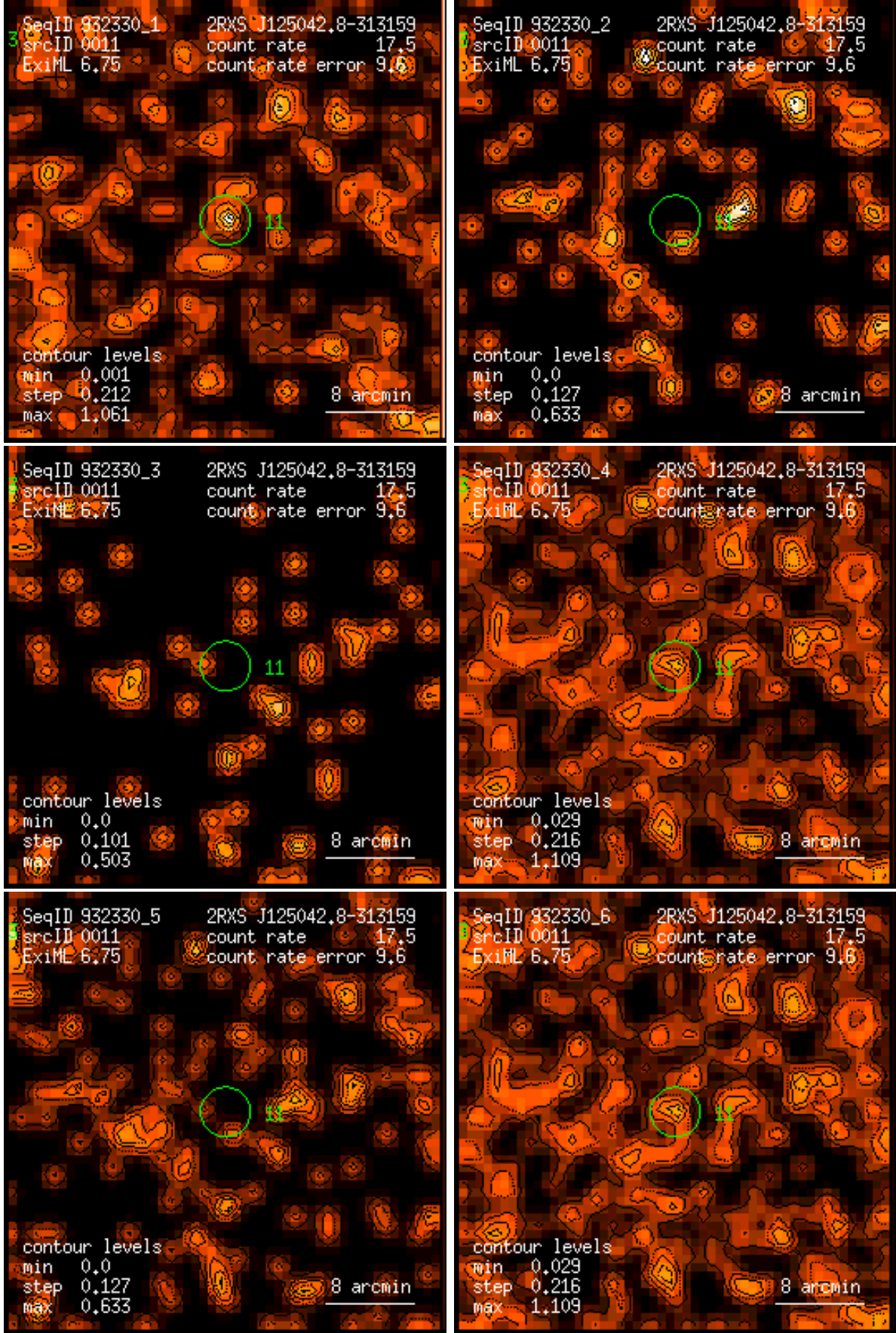
Figure 11: RASS 932330: detection 0011: band rate images, Gaussian filter: (1) PSPC channels 11 – 41, (2) 52 – 90, (3) 91 – 201, (4) 11 – 235, (5) 52 – 201, (6) 11 – 201. Broad band rates in counts/ks. Band rate contour levels in counts/ks/arcmin 2 .
