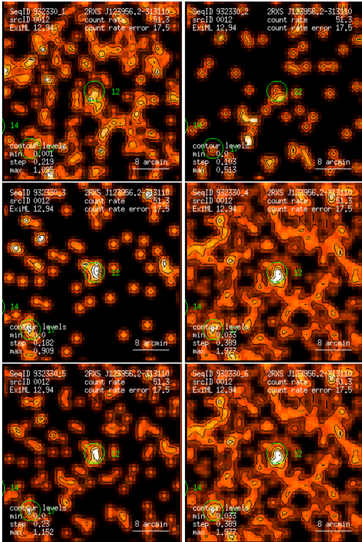
Figure 12: RASS 932330: detection 0012: band rate images, Gaussian filter: (1) PSPC channels 11 – 41, (2) 52 – 90, (3) 91 – 201, (4) 11 – 235, (5) 52 – 201, (6) 11 – 201. Broad band rates in counts/ks. Band rate contour levels in counts/ks/arcmin 2 .
