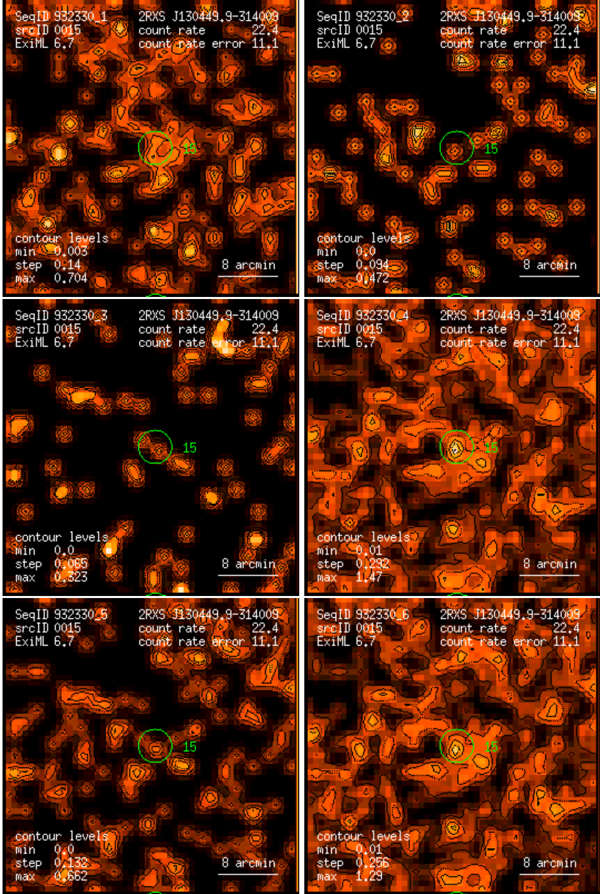
Figure 15: RASS 932330: detection 0015: band rate images, Gaussian filter: (1) PSPC channels 11 – 41, (2) 52 – 90, (3) 91 – 201, (4) 11 – 235, (5) 52 – 201, (6) 11 – 201. Broad band rates in counts/ks. Band rate contour levels in counts/ks/arcmin 2 .
