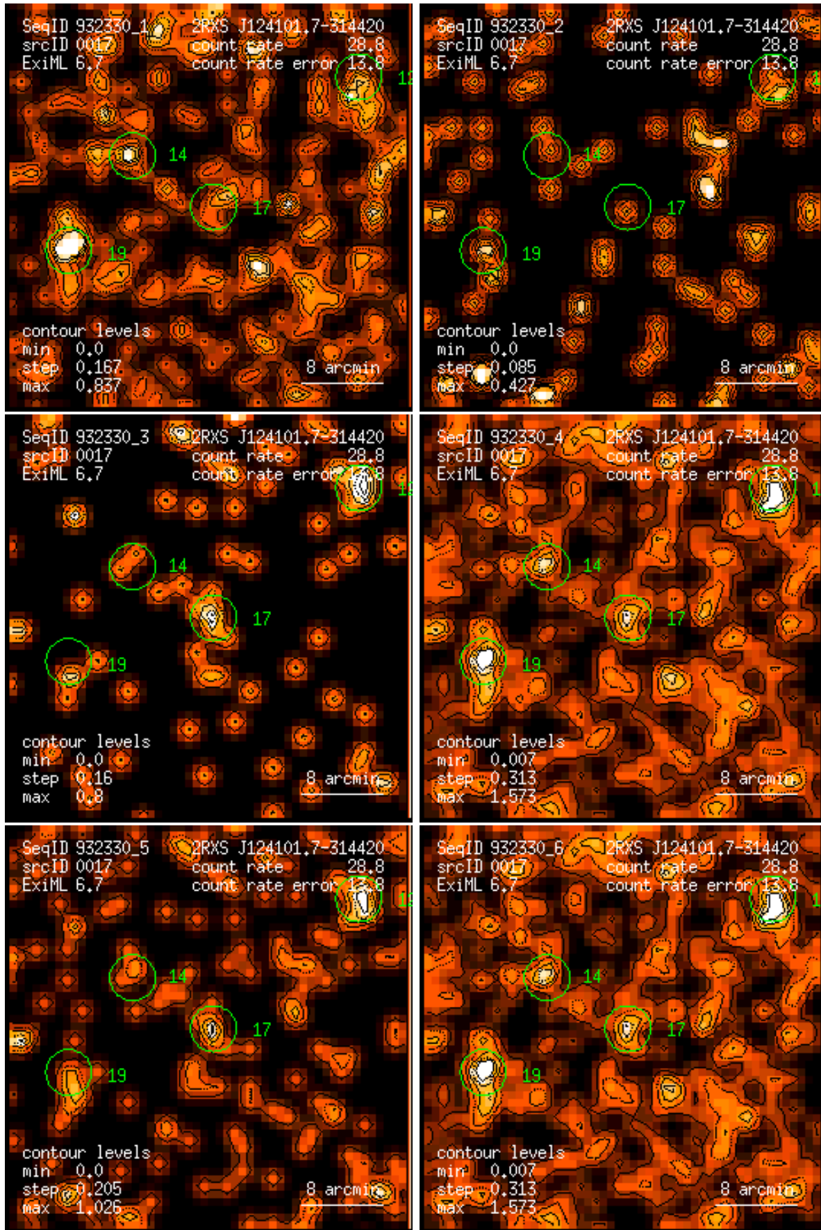
Figure 17: RASS 932330: detection 0017: band rate images, Gaussian filter: (1) PSPC channels 11 – 41, (2) 52 – 90, (3) 91 – 201, (4) 11 – 235, (5) 52 – 201, (6) 11 – 201. Broad band rates in counts/ks. Band rate contour levels in counts/ks/arcmin 2 .
