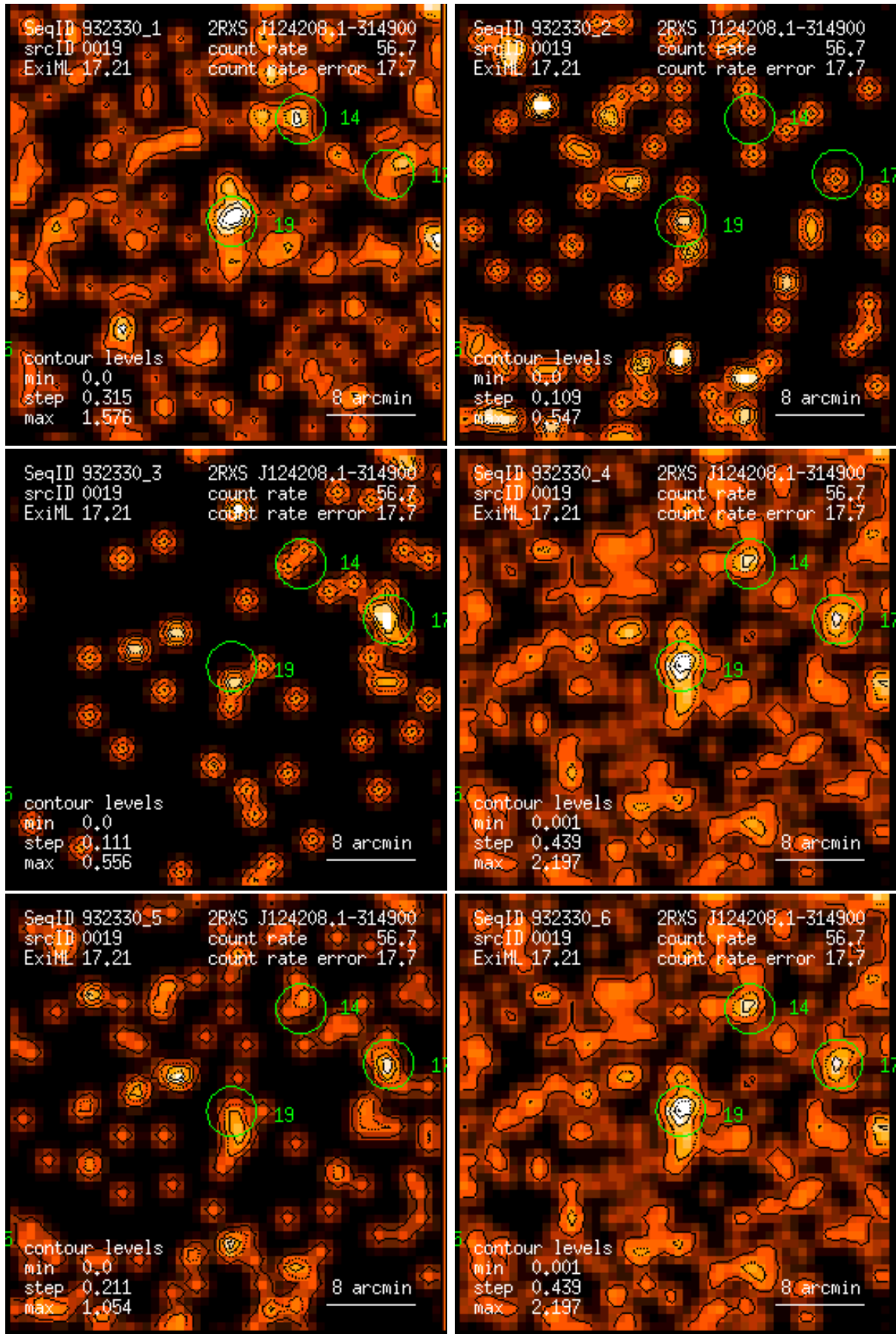
Figure 19: RASS 932330: detection 0019: band rate images, Gaussian filter: (1) PSPC channels 11 – 41, (2) 52 – 90, (3) 91 – 201, (4) 11 – 235, (5) 52 – 201, (6) 11 – 201. Broad band rates in counts/ks. Band rate contour levels in counts/ks/arcmin 2 .
