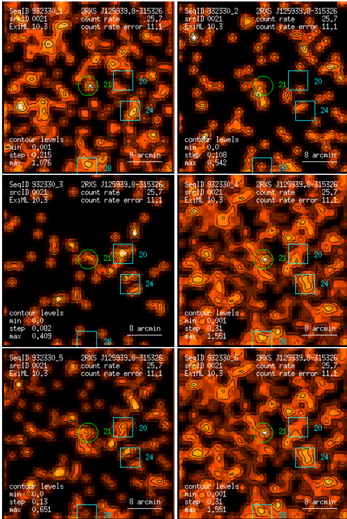
Figure 21: RASS 932330: detection 0021: band rate images, Gaussian filter: (1) PSPC channels 11 – 41, (2) 52 – 90, (3) 91 – 201, (4) 11 – 235, (5) 52 – 201, (6) 11 – 201. Broad band rates in counts/ks. Band rate contour levels in counts/ks/arcmin 2 .
