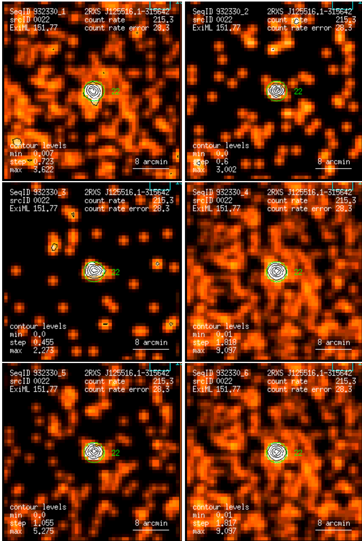
Figure 22: RASS 932330: detection 0022: band rate images, Gaussian filter: (1) PSPC channels 11 – 41, (2) 52 – 90, (3) 91 – 201, (4) 11 – 235, (5) 52 – 201, (6) 11 – 201. Broad band rates in counts/ks. Band rate contour levels in counts/ks/arcmin 2 .
