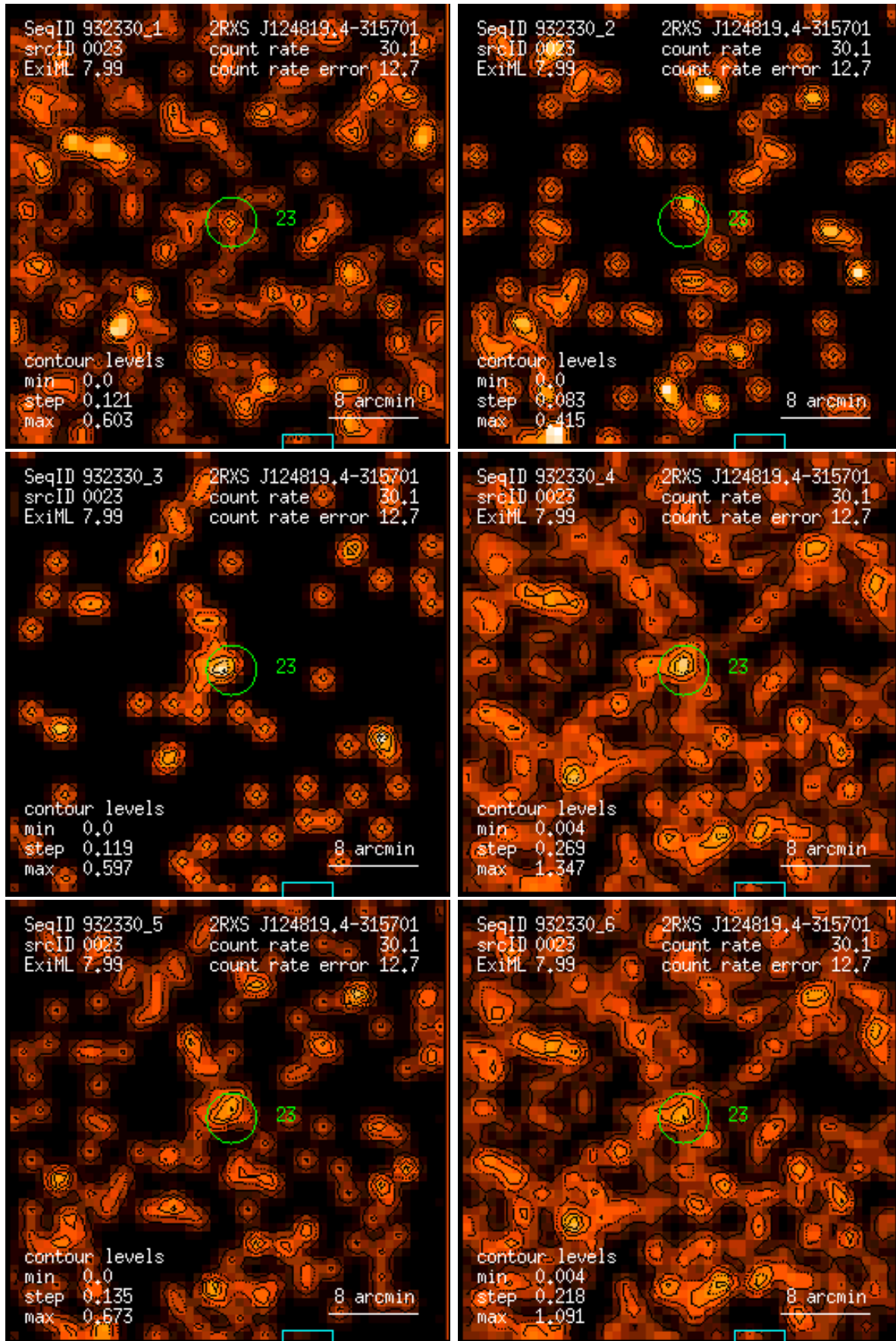
Figure 23: RASS 932330: detection 0023: band rate images, Gaussian filter: (1) PSPC channels 11 – 41, (2) 52 – 90, (3) 91 – 201, (4) 11 – 235, (5) 52 – 201, (6) 11 – 201. Broad band rates in counts/ks. Band rate contour levels in counts/ks/arcmin 2 .
