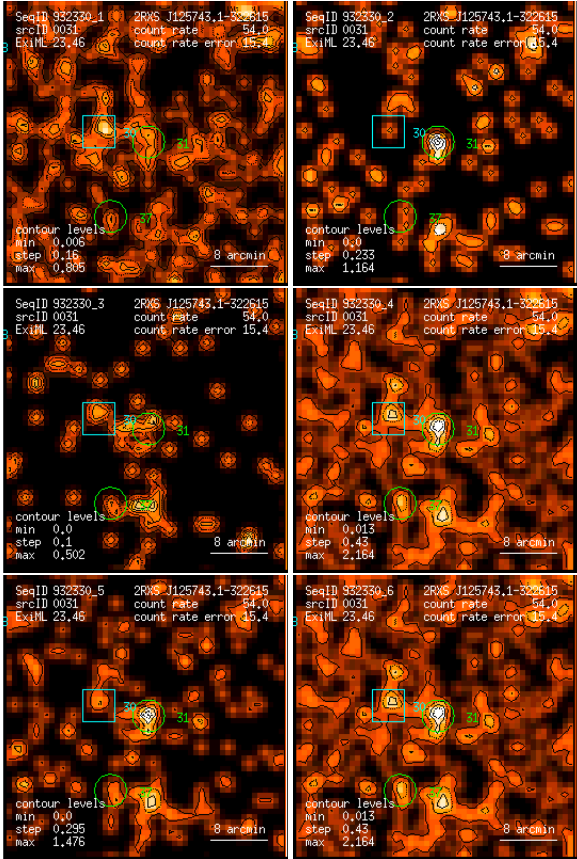
Figure 31: RASS 932330: detection 0031: band rate images, Gaussian filter: (1) PSPC channels 11 – 41, (2) 52 – 90, (3) 91 – 201, (4) 11 – 235, (5) 52 – 201, (6) 11 – 201. Broad band rates in counts/ks. Band rate contour levels in counts/ks/arcmin 2 .
