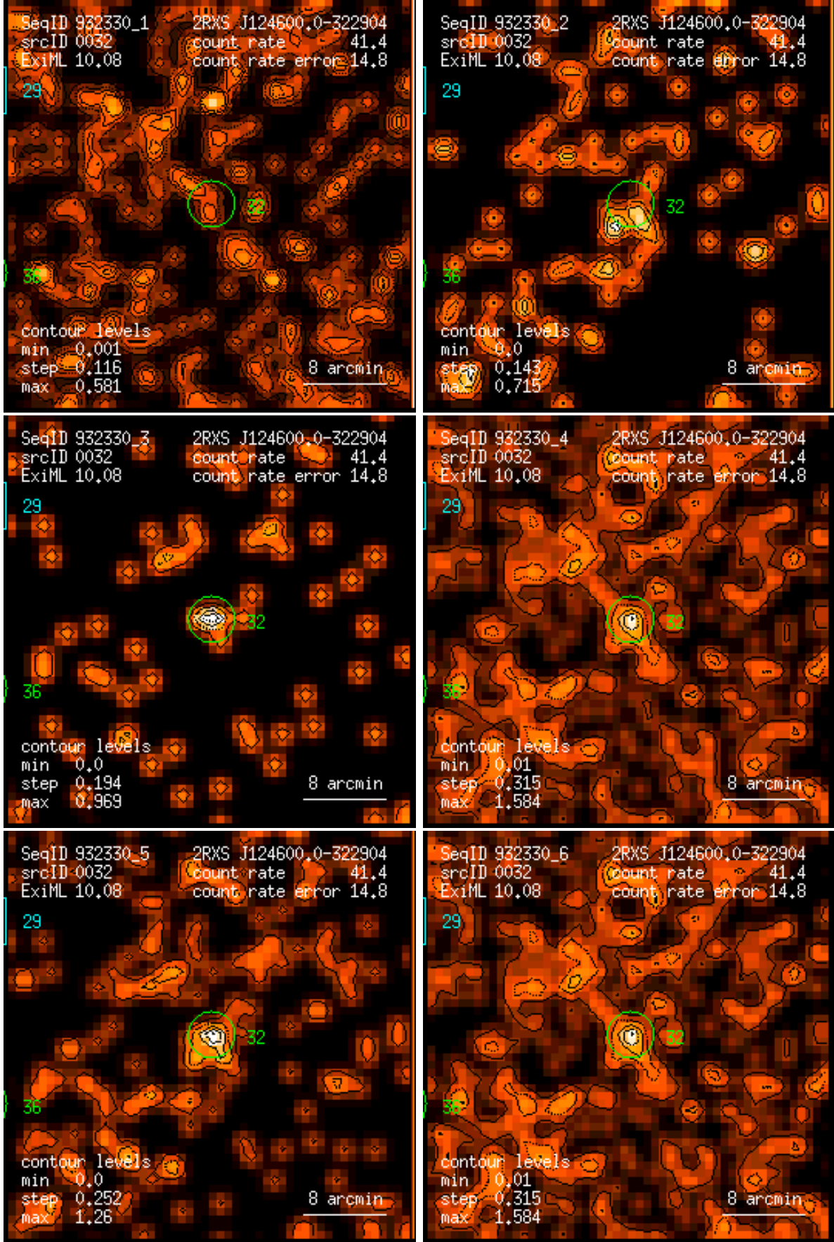
Figure 32: RASS 932330: detection 0032: band rate images, Gaussian filter: (1) PSPC channels 11 – 41, (2) 52 – 90, (3) 91 – 201, (4) 11 – 235, (5) 52 – 201, (6) 11 – 201. Broad band rates in counts/ks. Band rate contour levels in counts/ks/arcmin 2 .
